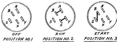
REAR VIEW OF IGNITION SWITCH
