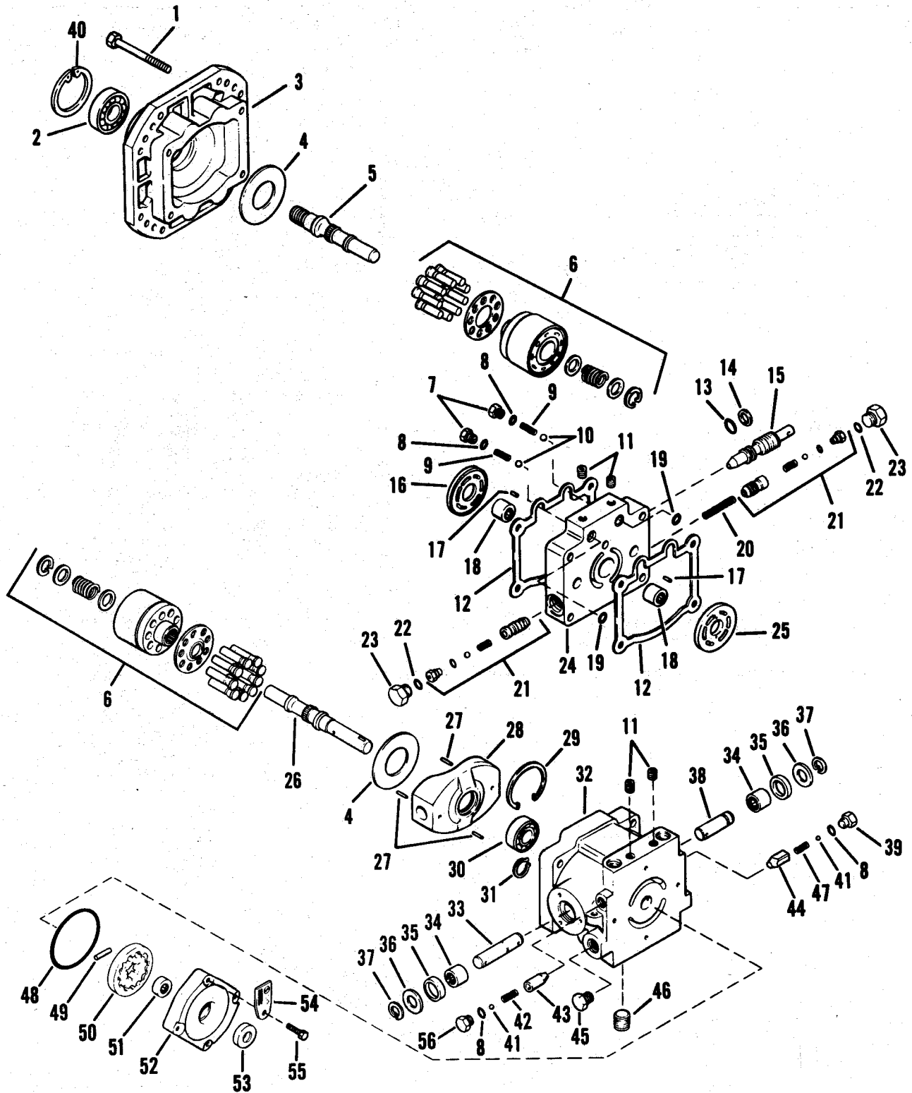
Figure 3A. HYDRO ASSEMBLY
