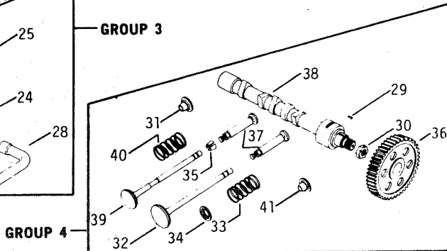
Figure 2A KOHLER ENGINE ASSEMBLY (K582S-36272A) KOHLER ENGINE ASSEMBLY (K582S-36328)
