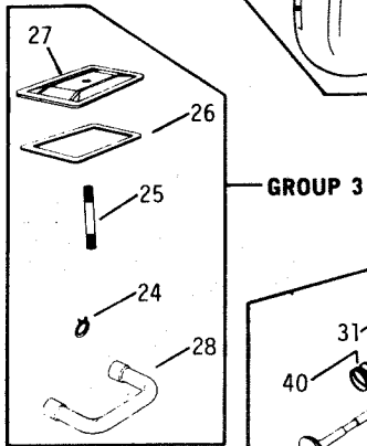
Figure 2A KOHLER ENGINE ASSEMBLY (K582S-36272A) KOHLER ENGINE ASSEMBLY (K582S-36328)
