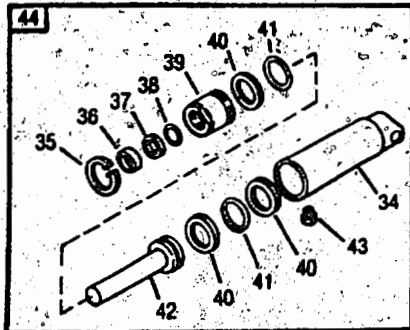
HYDROSTATIC & LIFT ASSEMBLY
