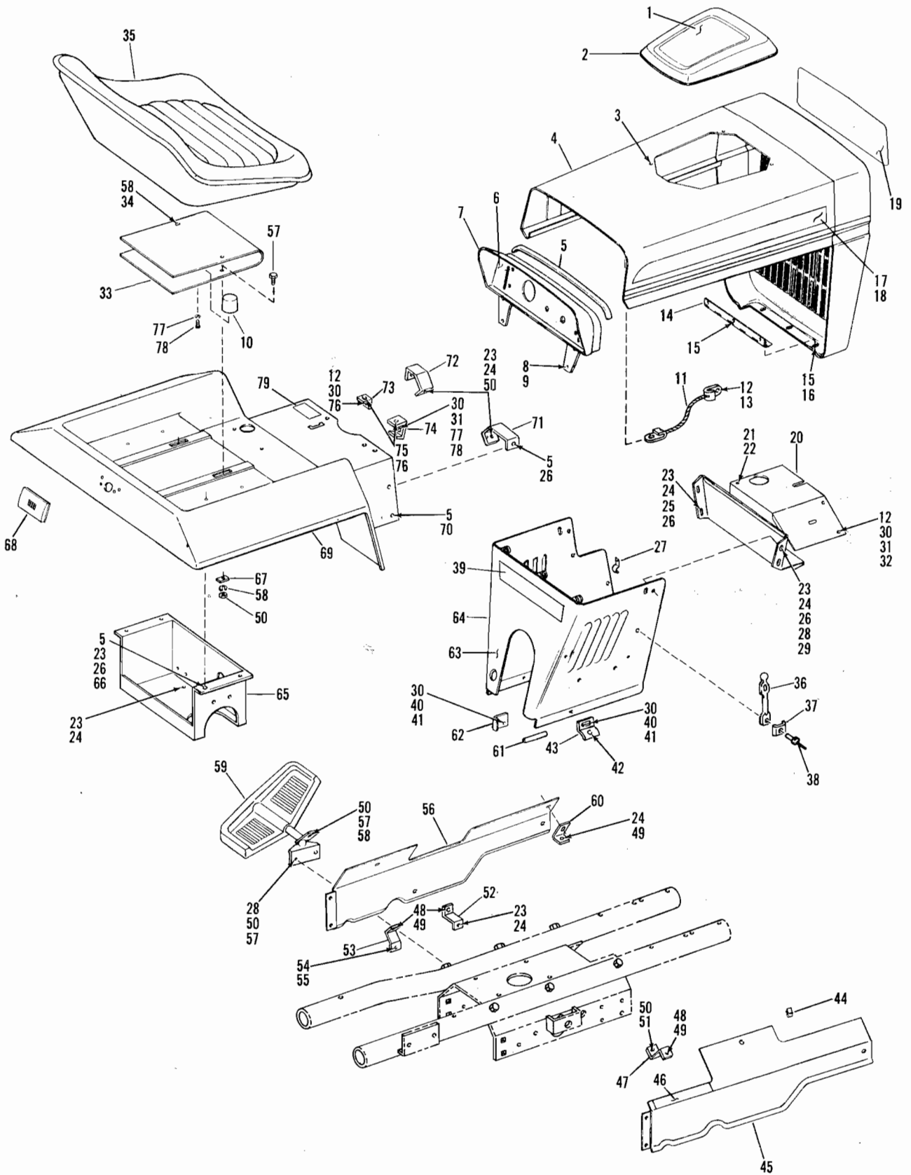
Figure 1 TRIM ASSEMBLY
