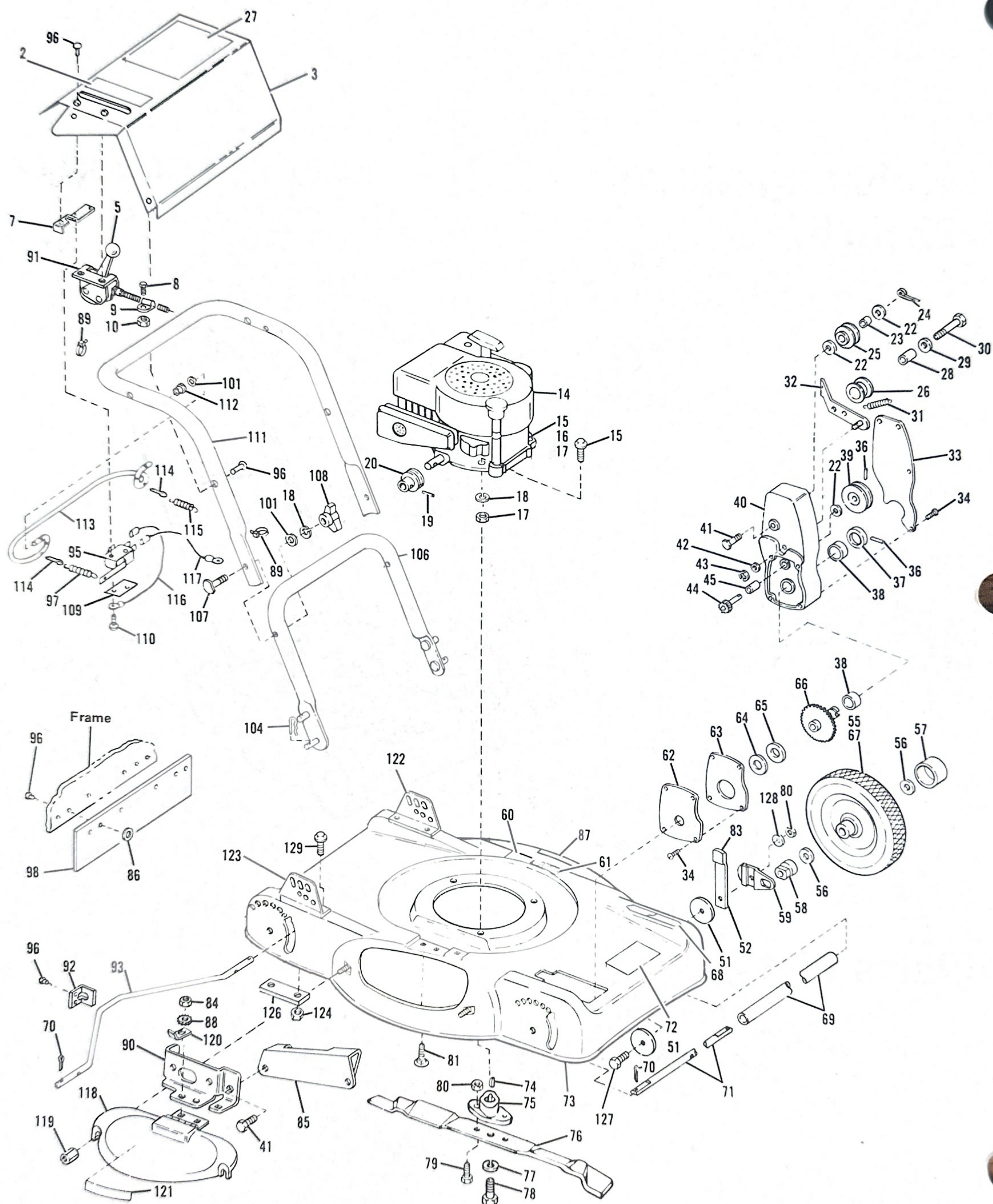
Figure 1 COMPLETE ASSEMBLY
