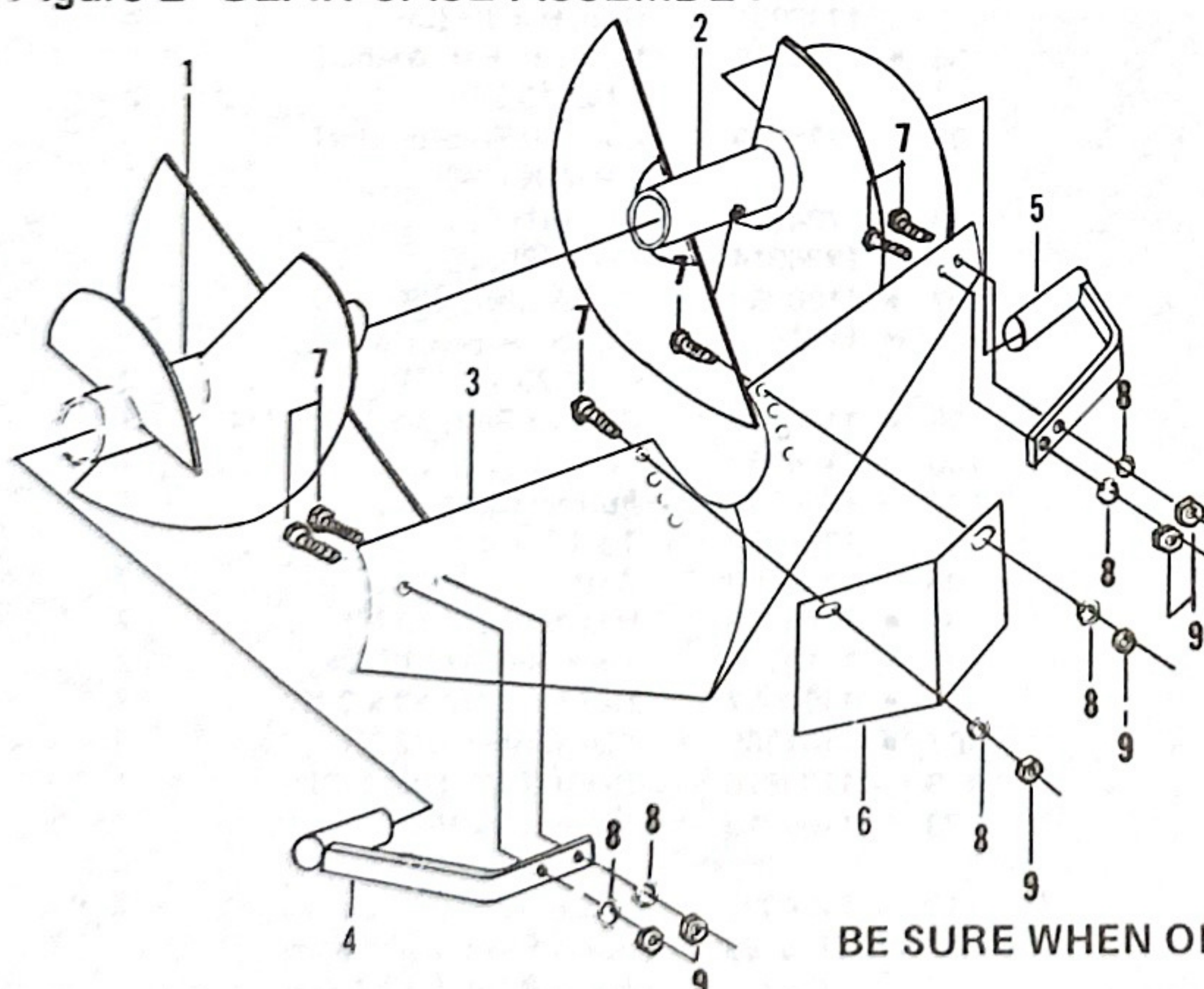
Figure 3 MODEL 6868 TIL-ROW ATTACHMENT (Optional)
