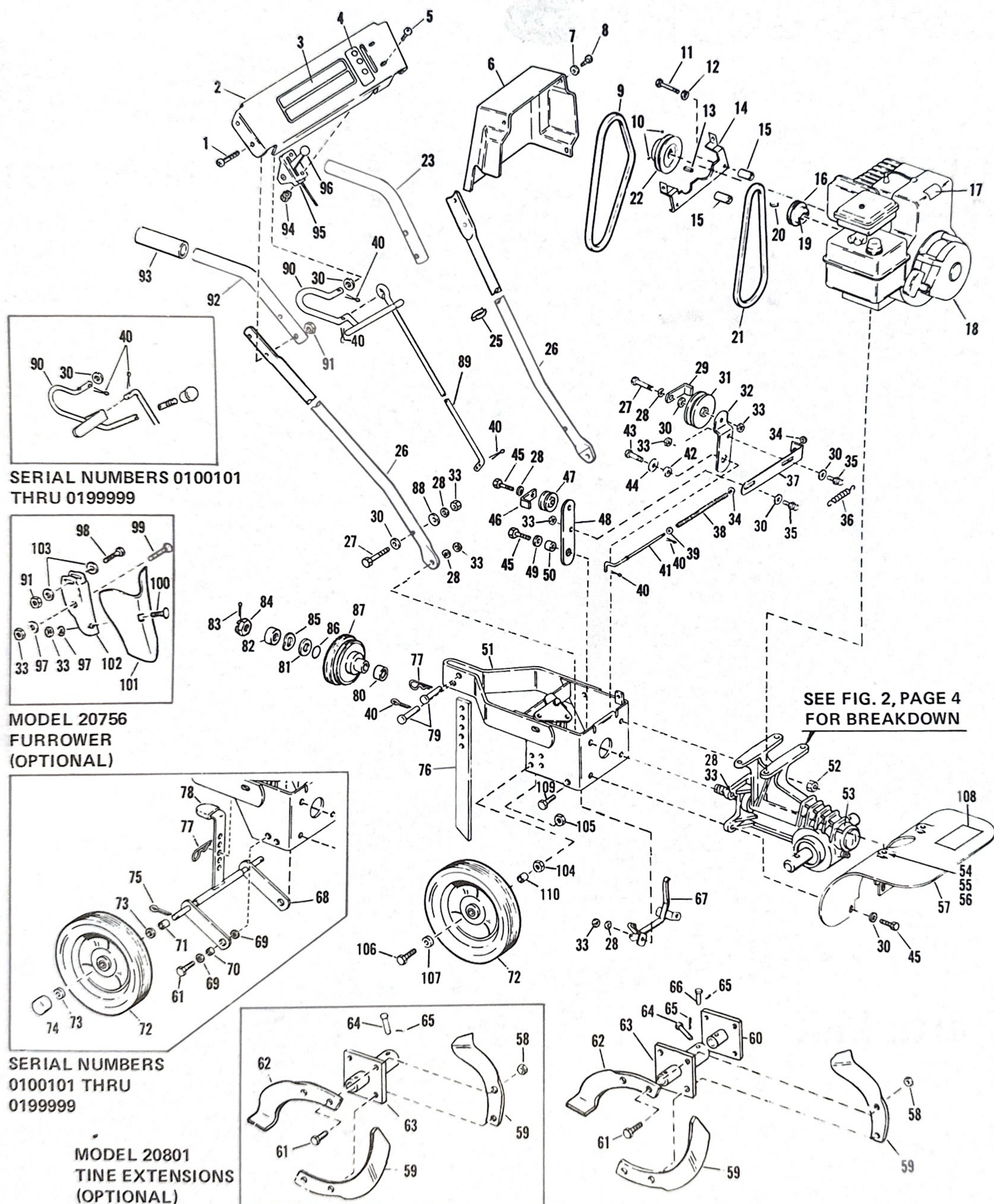
Figure 1 COMPLETE ASSEMBLY
