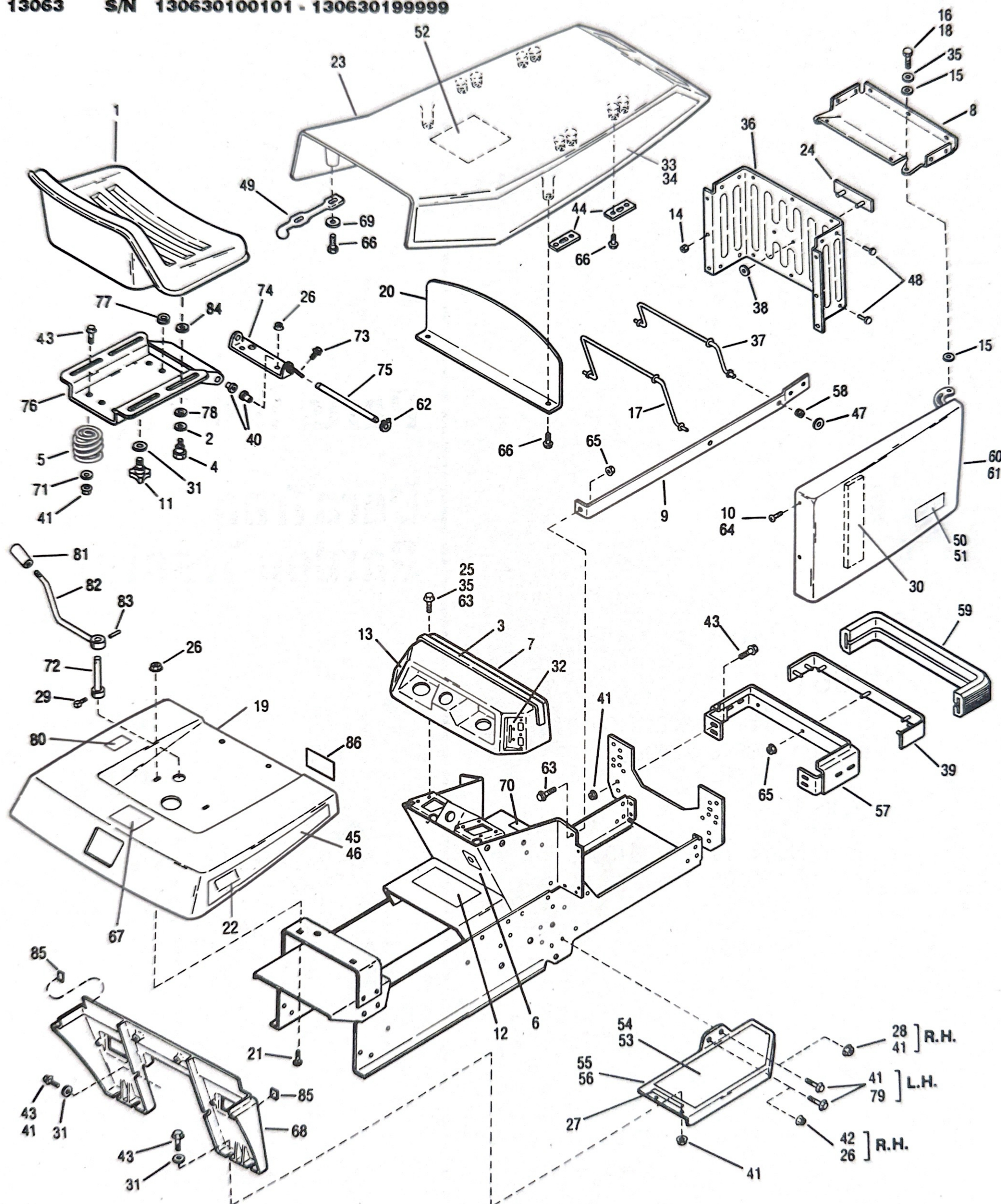
BODY AND TRIM ASSEMBLY
