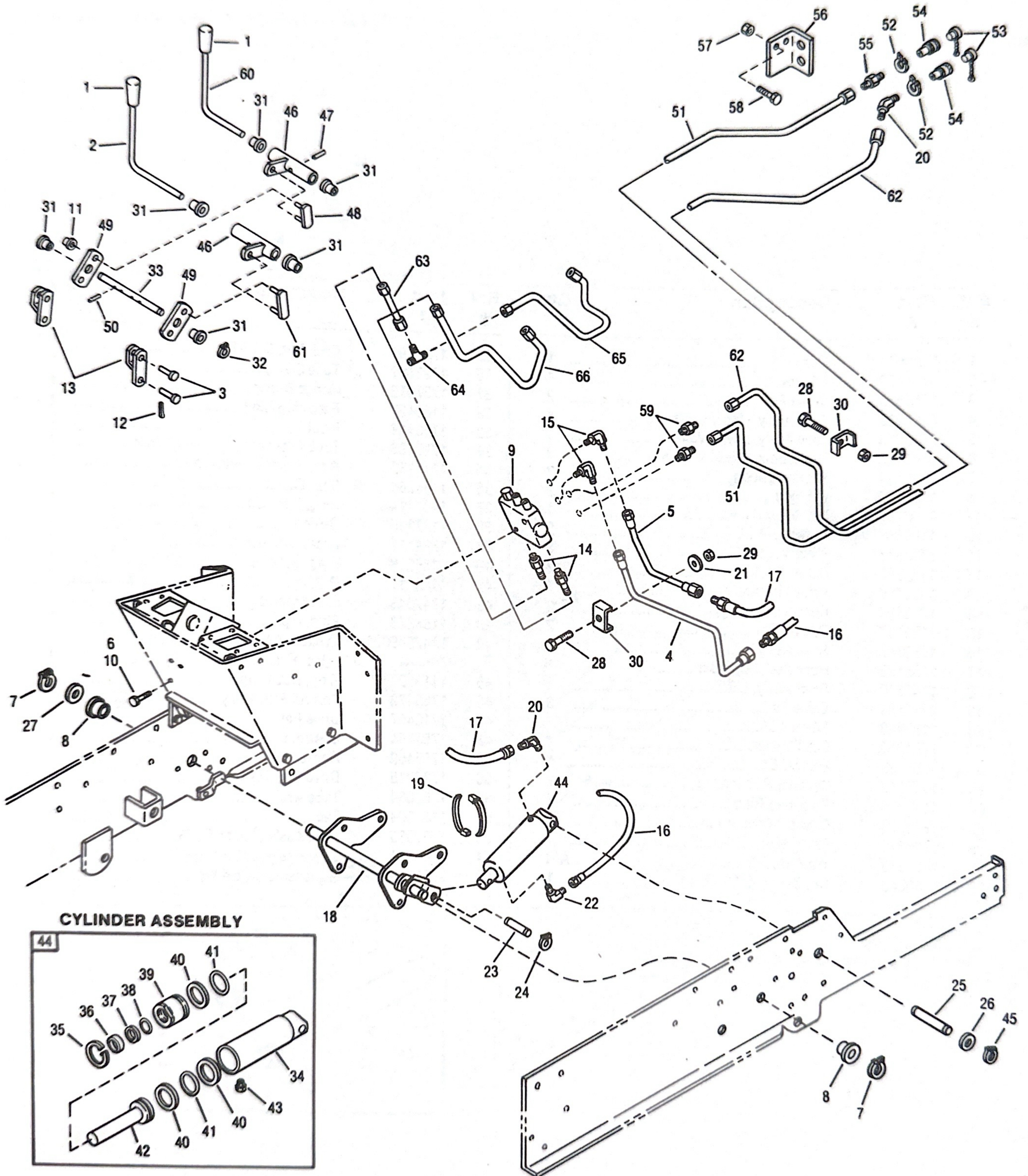
LIFT ASSEMBLY
