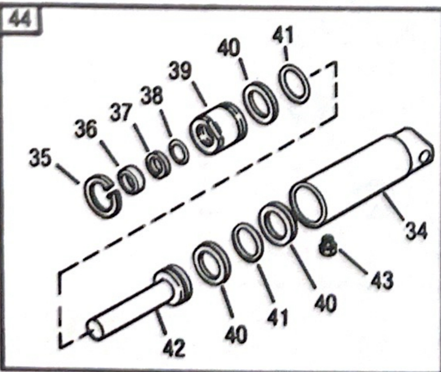
CYLINDER ASSEMBLY
