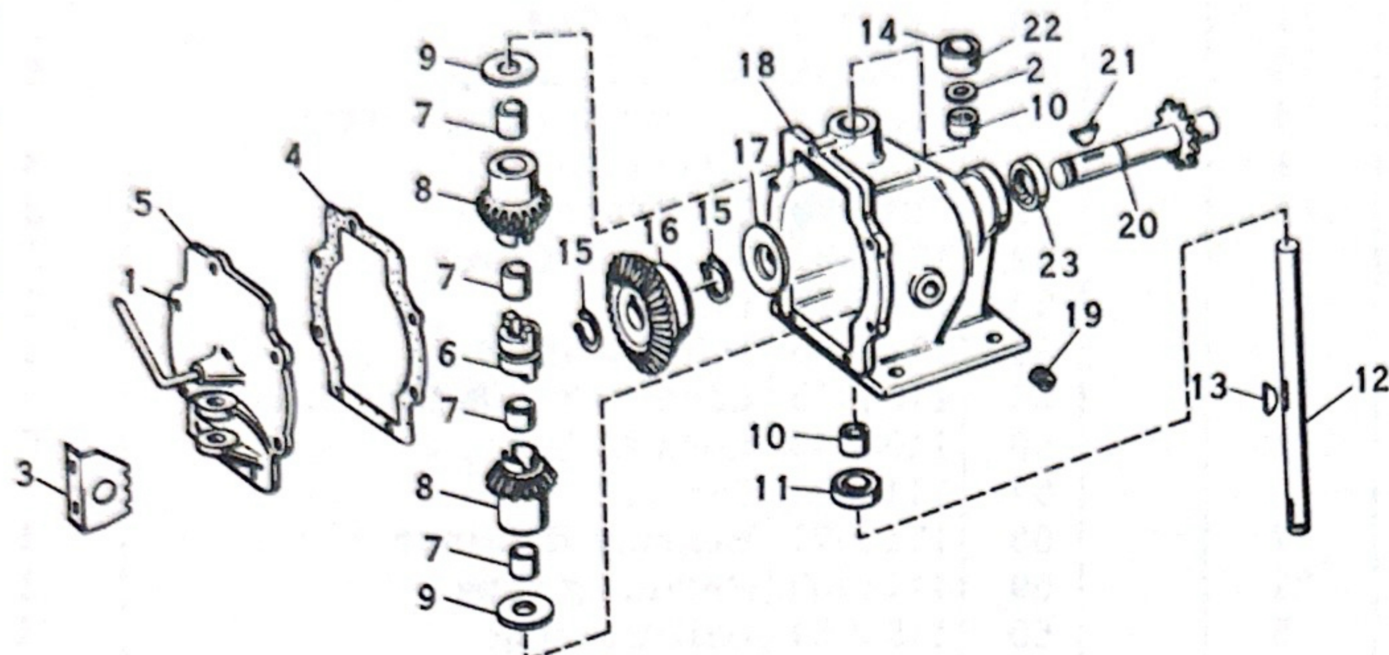
Figure 2. Gear Case Assembly
