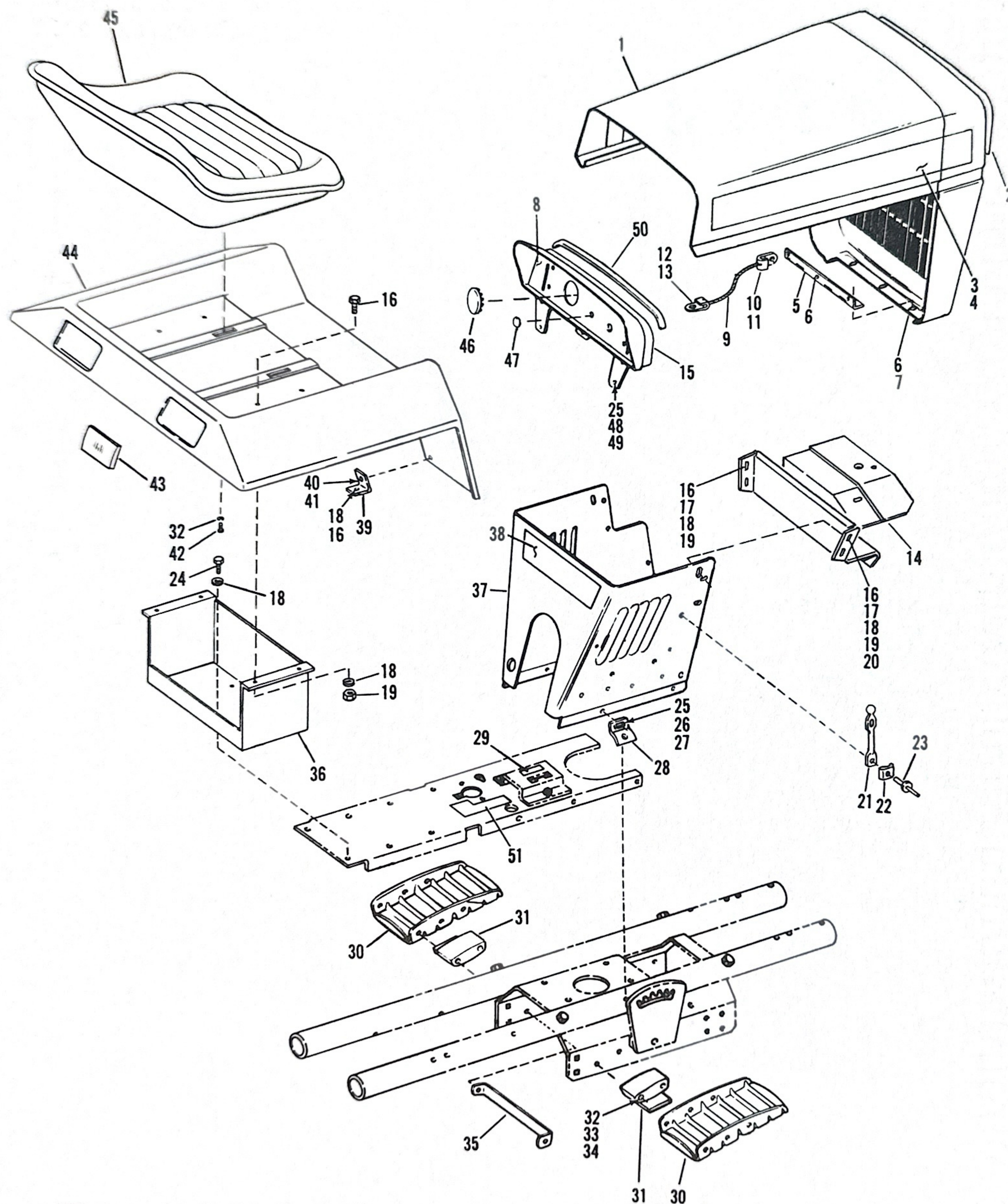
Figure 1. TRIM ASSEMBLY
