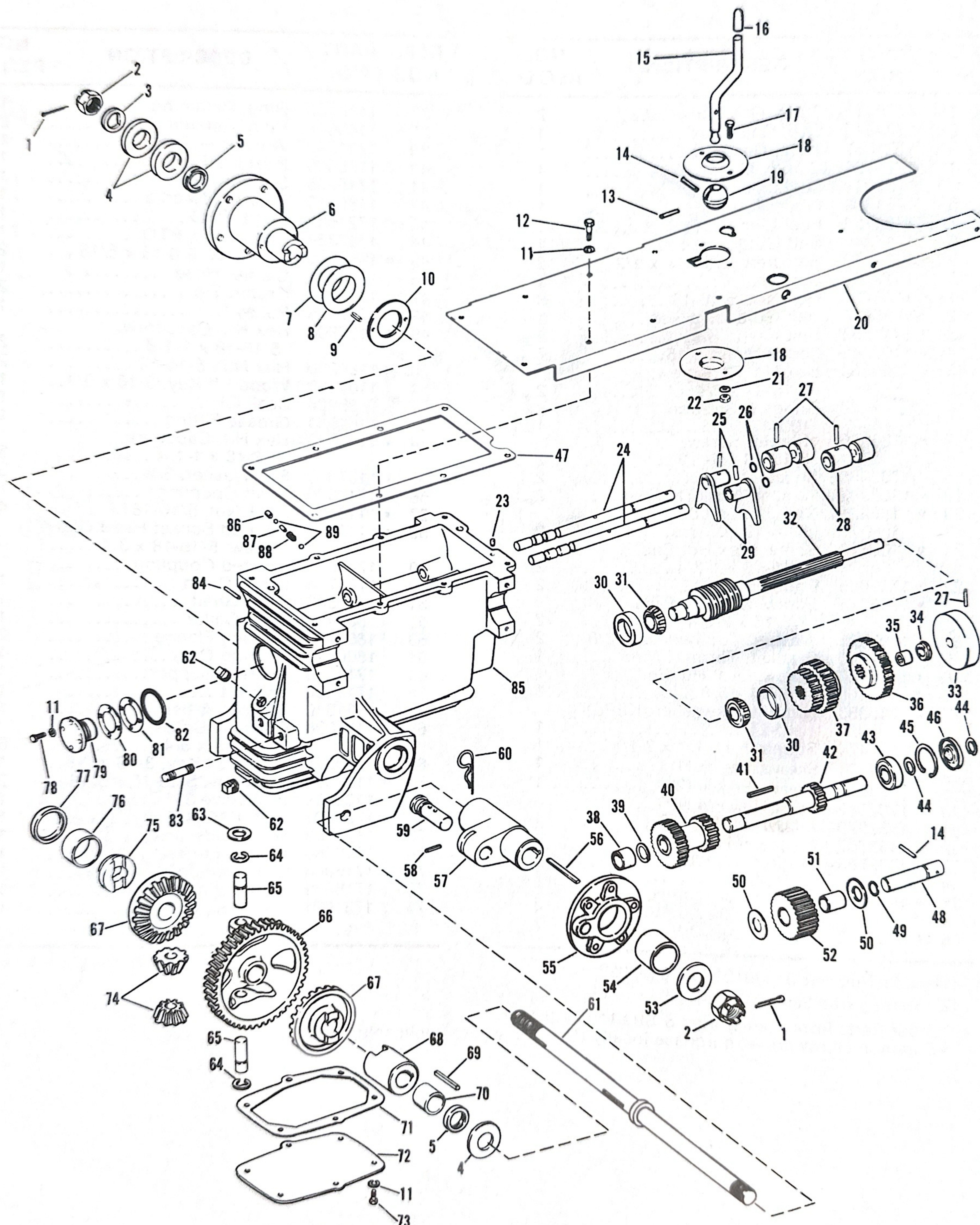
Figure 3. TRANSMISSION ASSEMBLY
