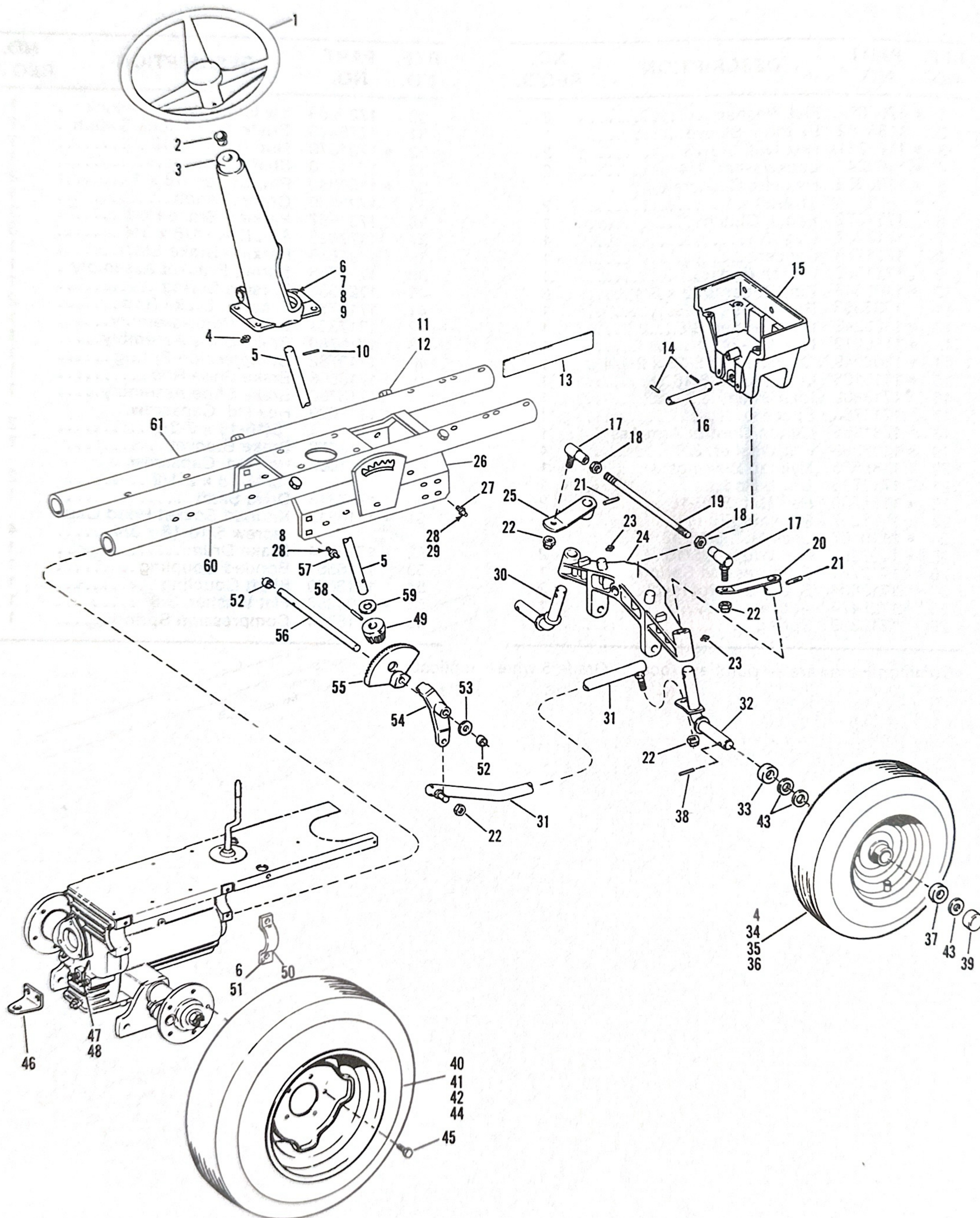
Figure 6. FRAME, STEERING and AXLE ASSEMBLIES
