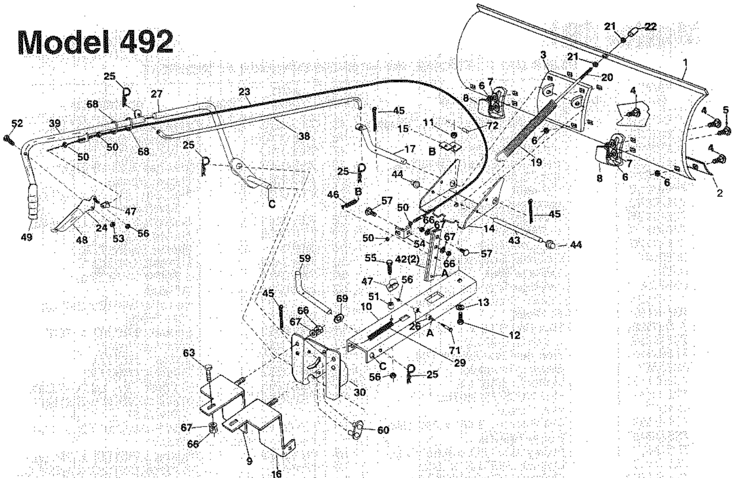
PARTS LIST FOR MODEL 190-492 42" SNOW BLADE
