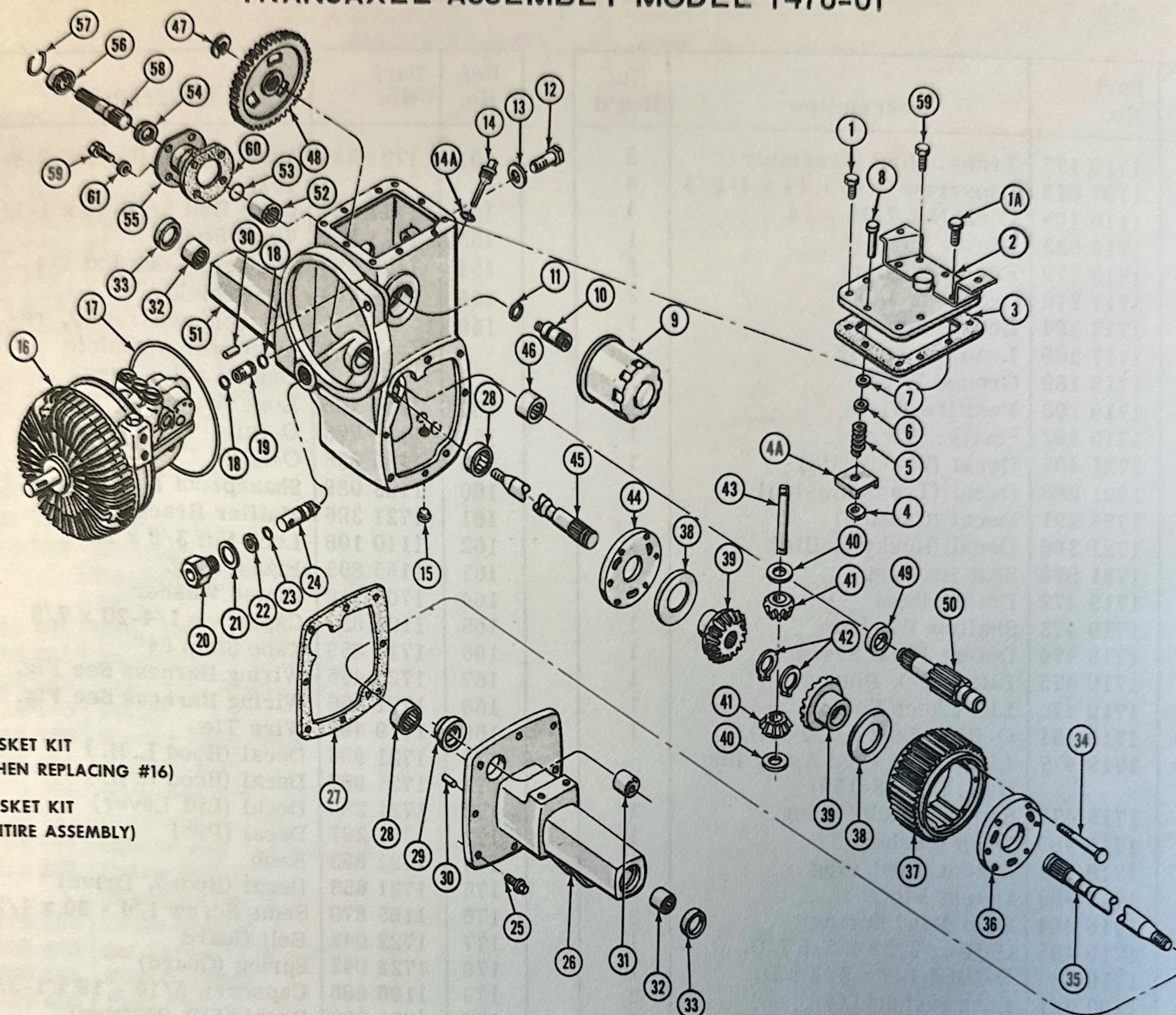
Parts List For Figure 8
