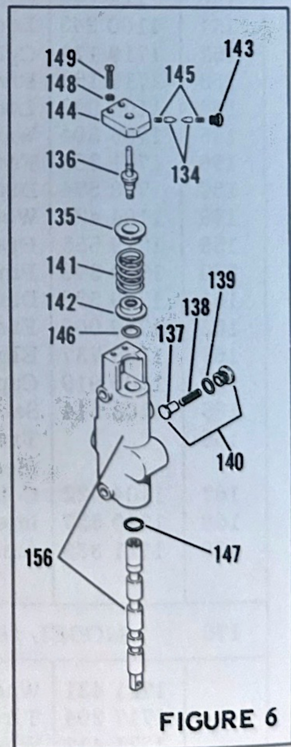
CONTROL VALVE ASS'Y. (REF. NO. 62)
