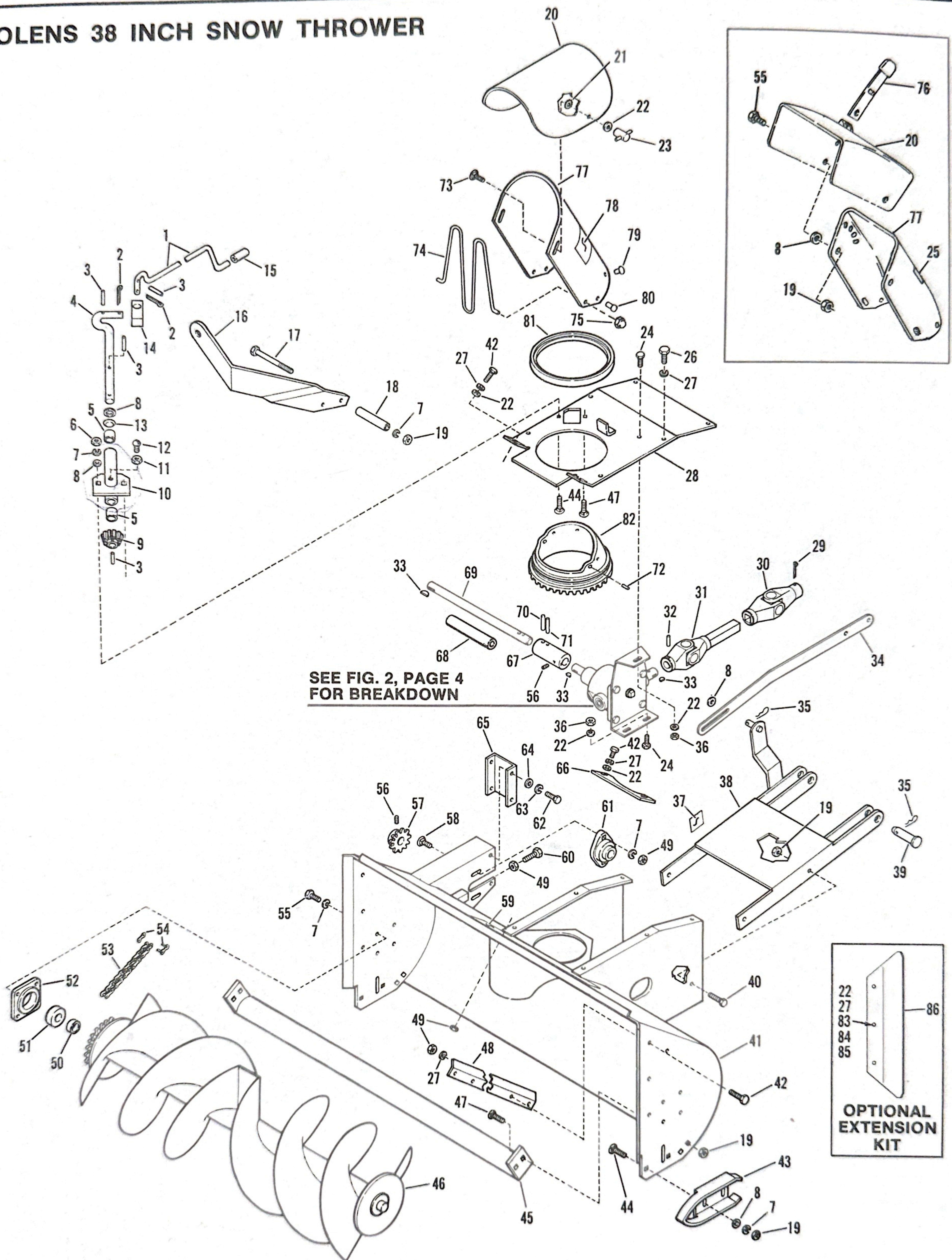
Figure 1 COMPLETE ASSEMBLY
