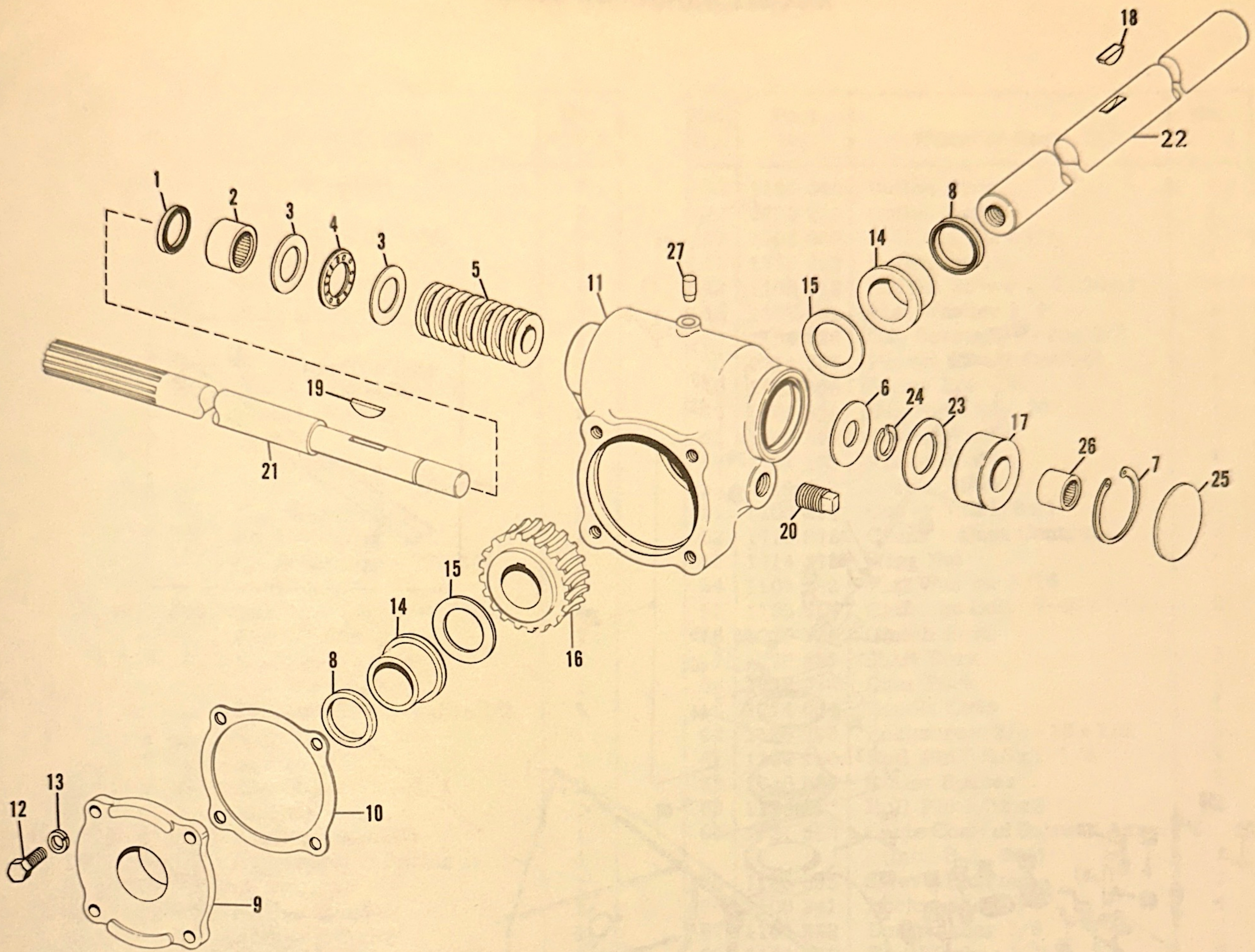
Figure 2, GEAR CASE ASSEMBLY
