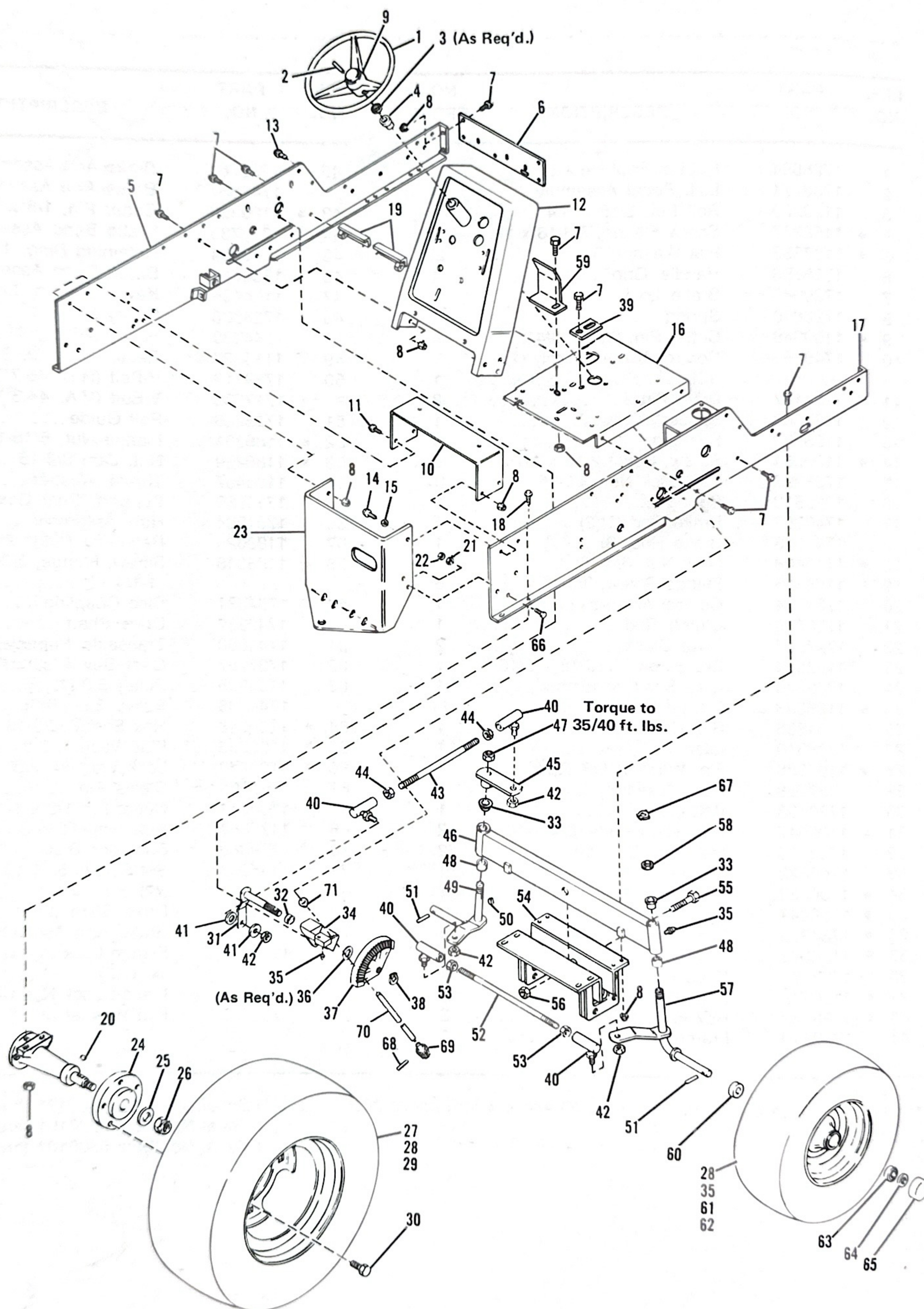
Figure 4. FRAME STEERING AND AXLE ASSEMBLIES
