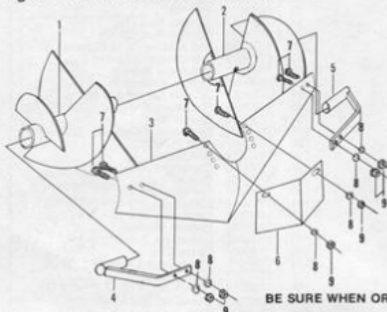
Figure 3 MODEL 6868 TIL-ROW ATTACHMENT (Optional)
