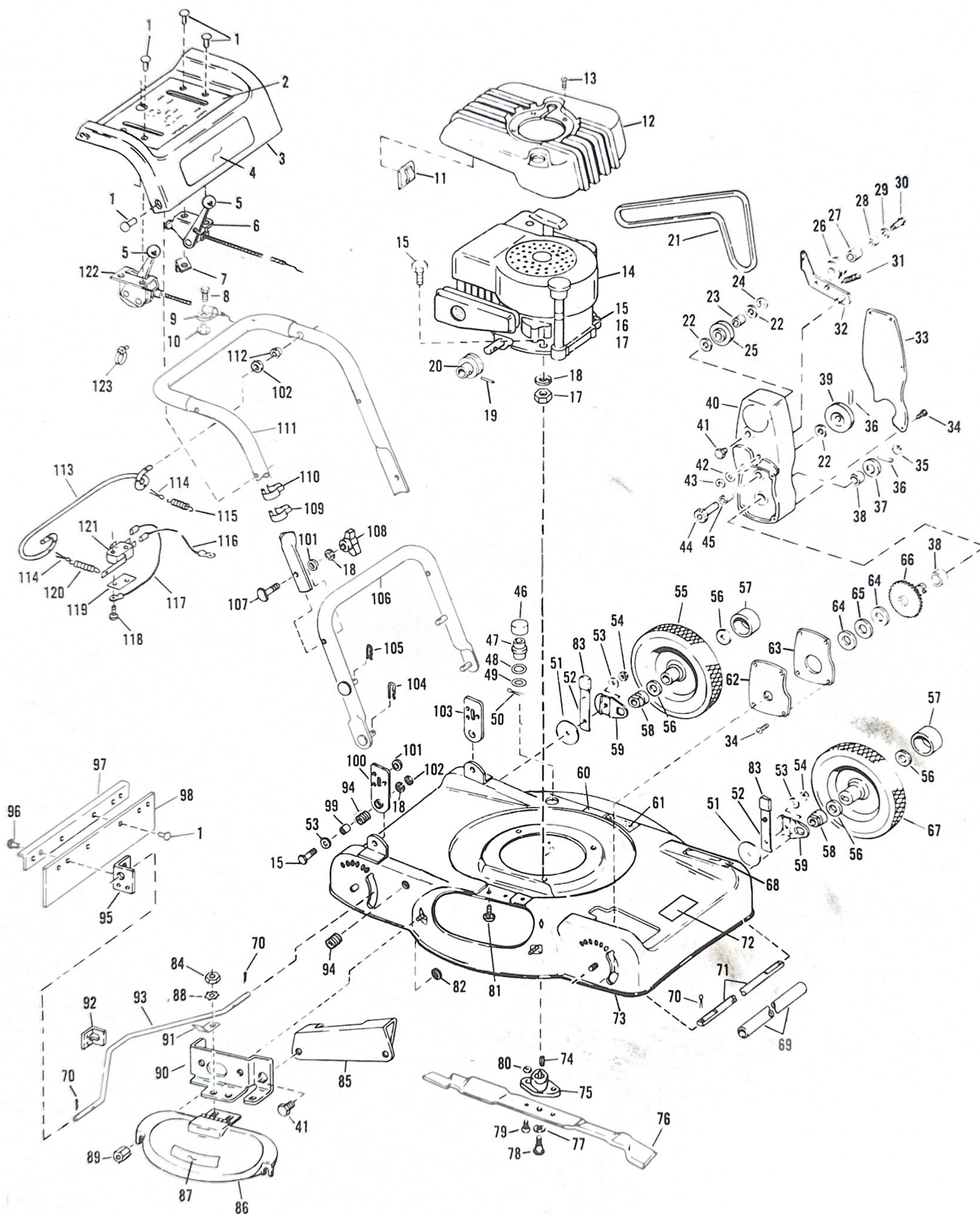
Figure 1 COMPLETE ASSEMBLY
