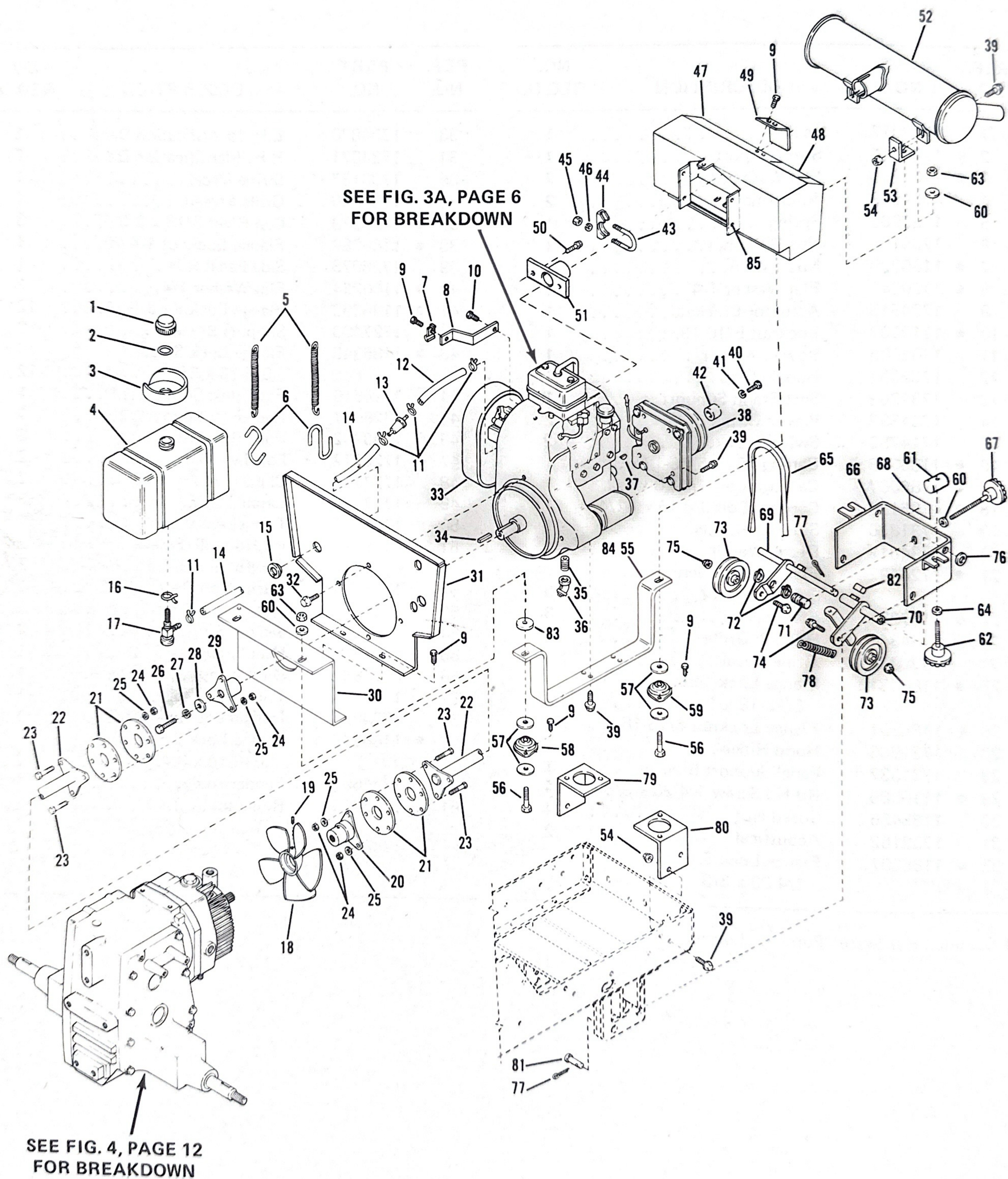
Figure 2. ENGINE AND DRIVE ASSEMBLY
