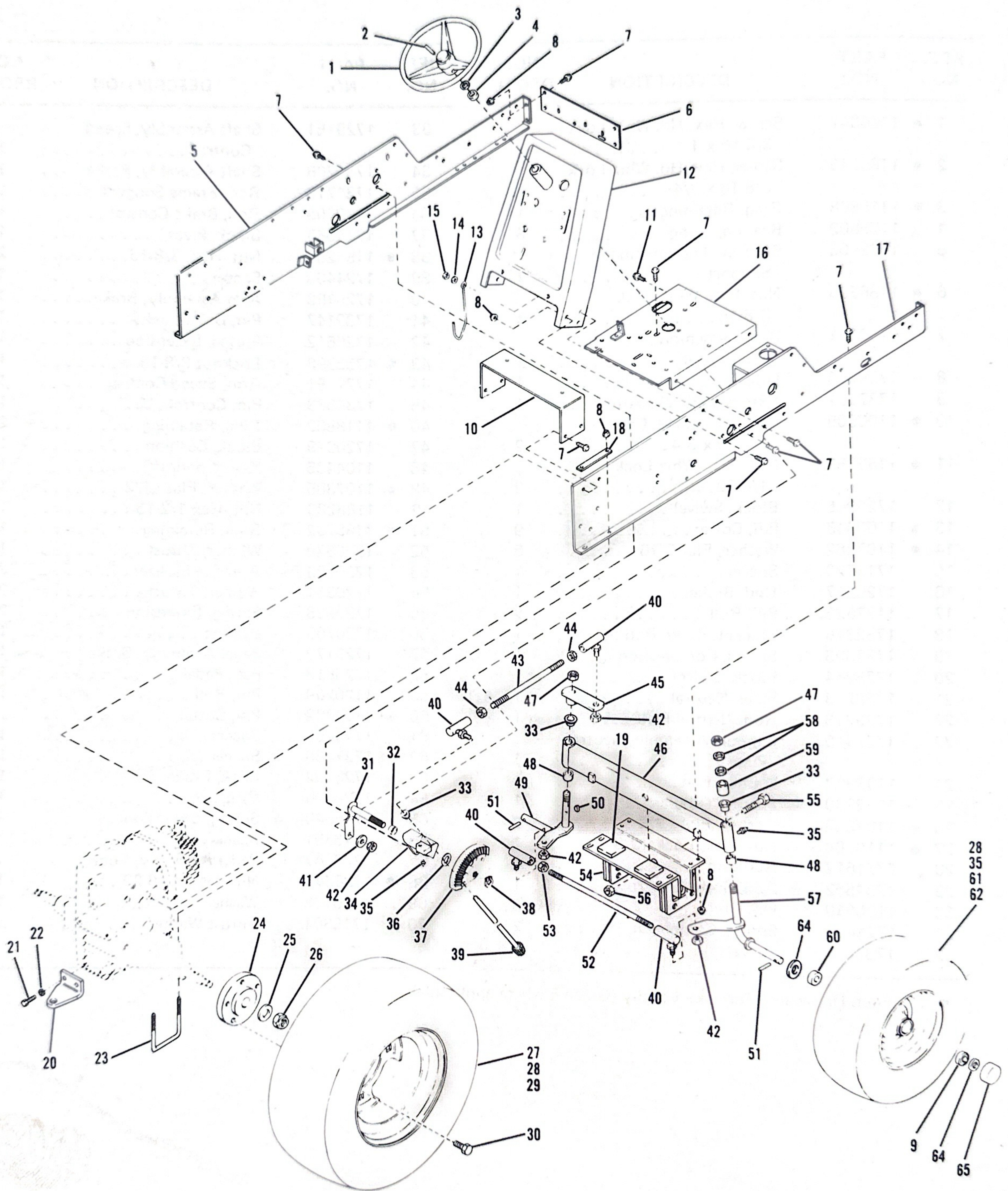
Figure 7. FRAME STEERING AND AXLE ASSEMBLIES
