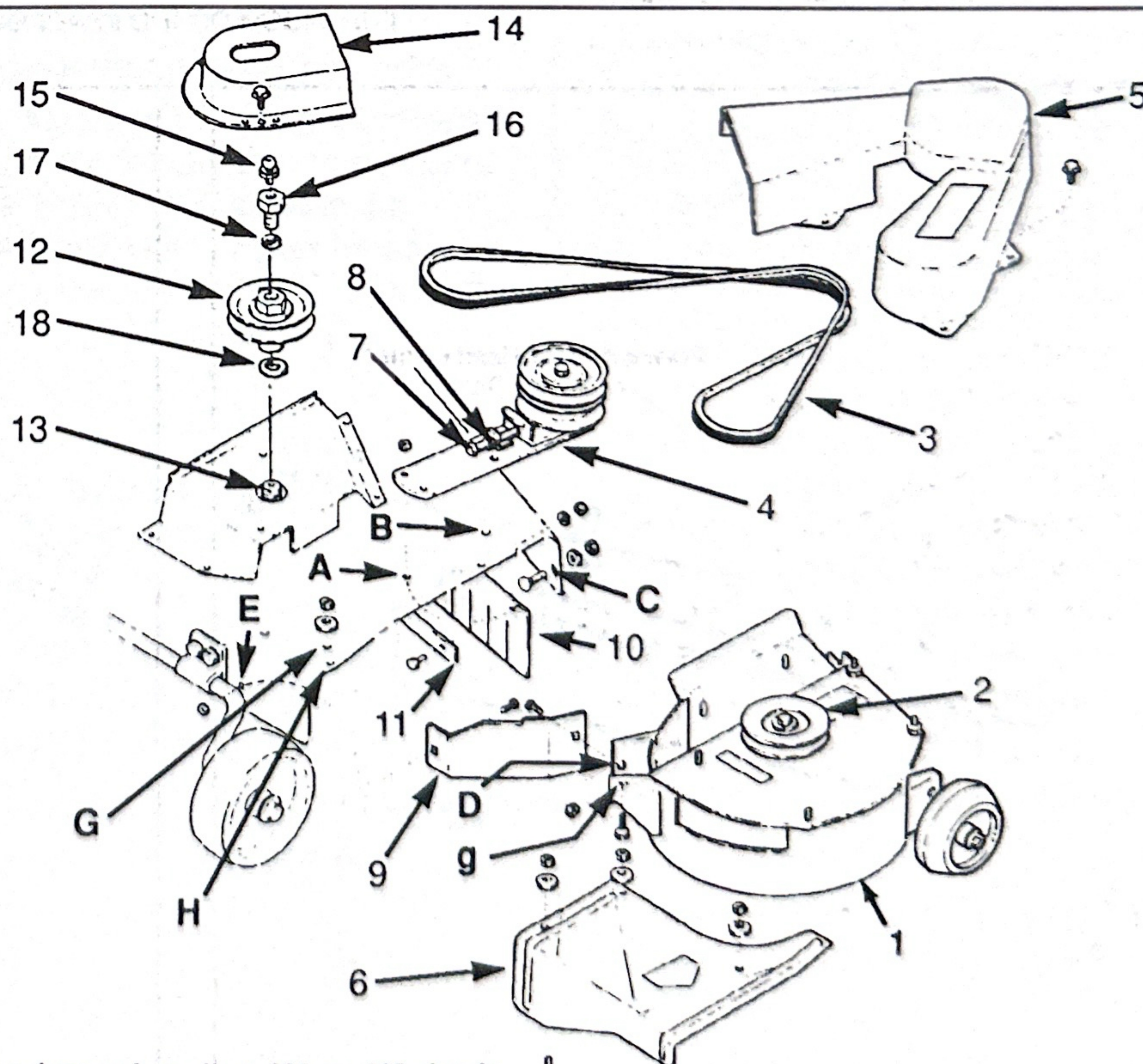
Fig. 2: Installing the Model 14011 Mulching Attachment on the 42" or 48" deck.
