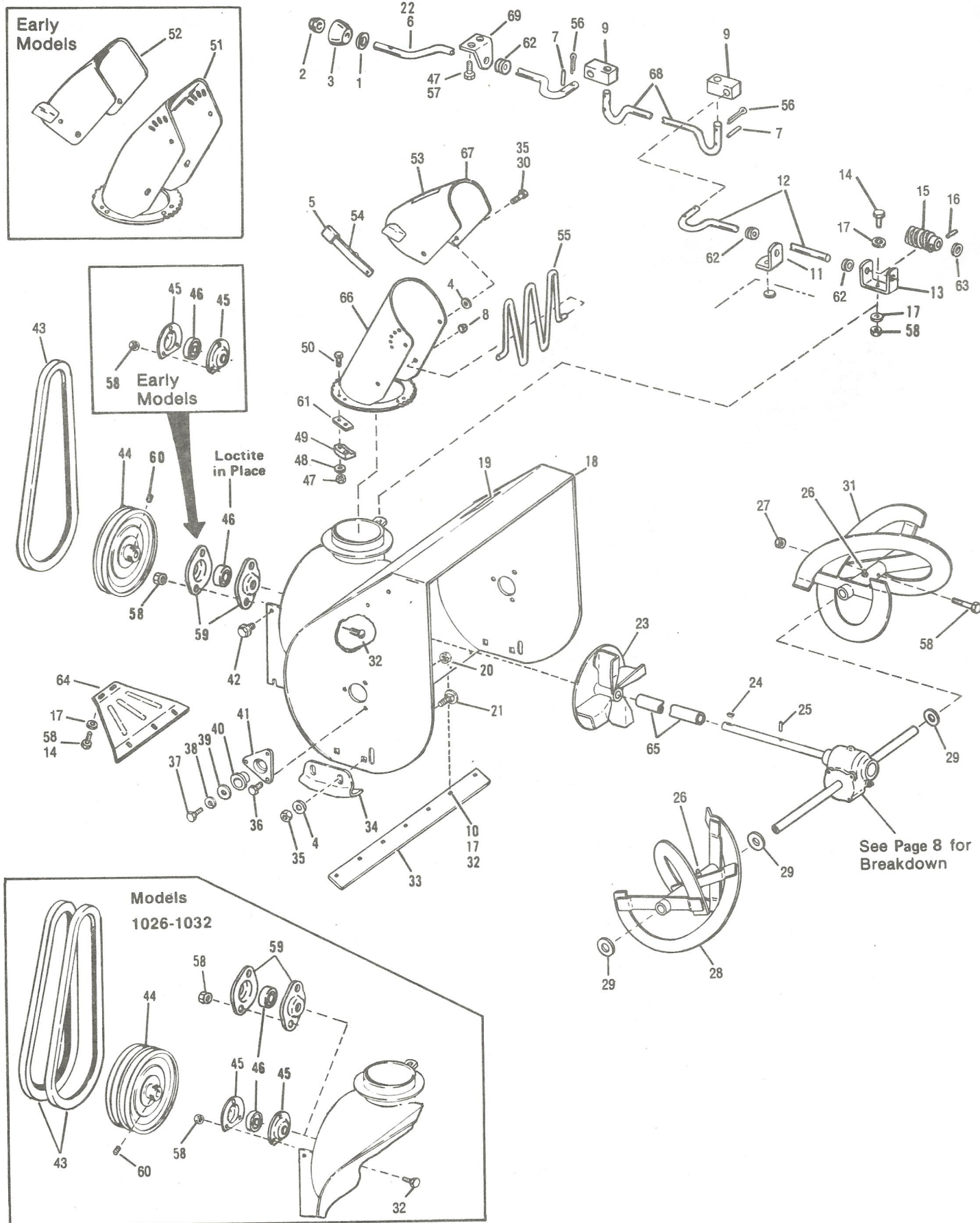
Figure 3 BLOWER HOUSING ASSEMBLY
