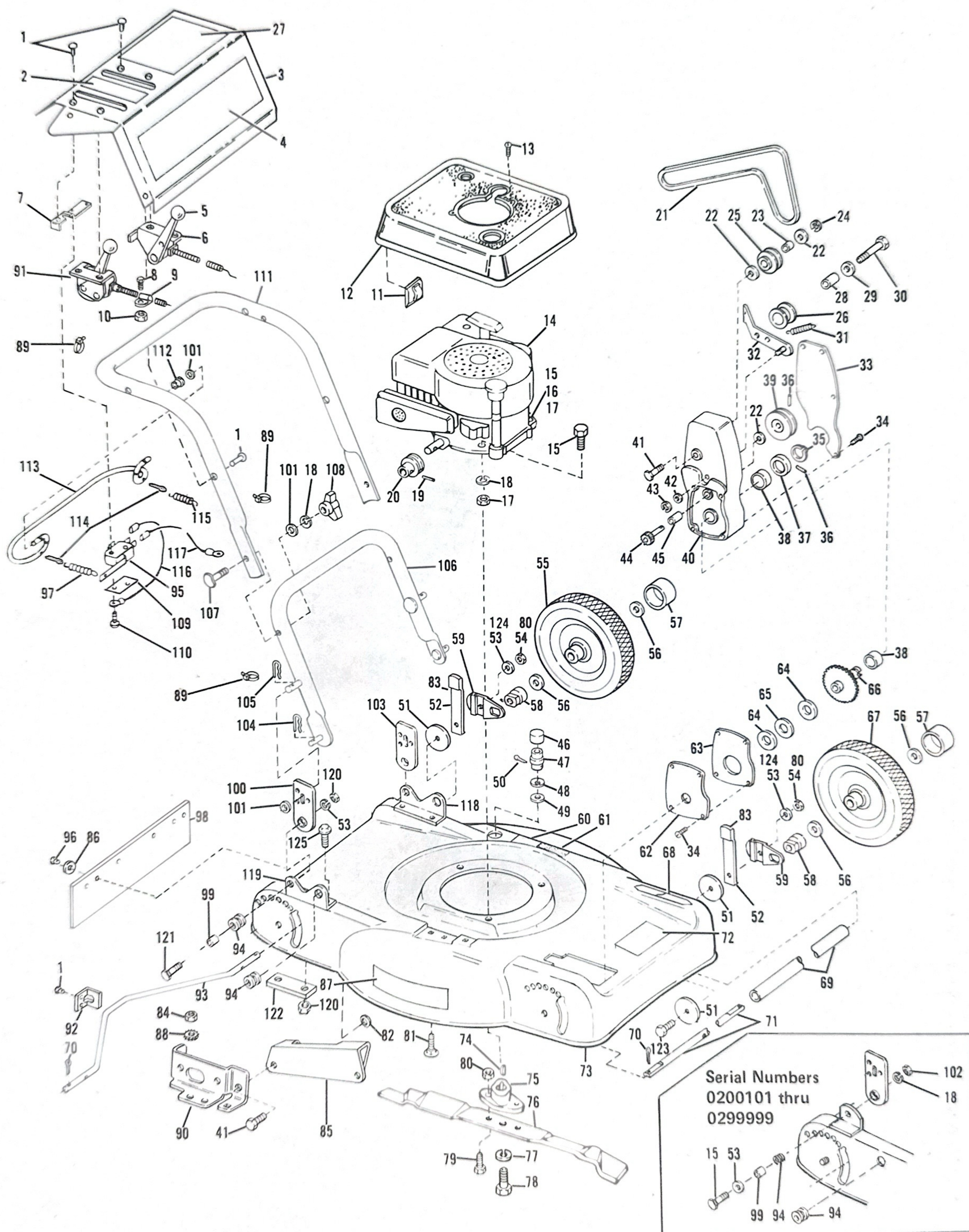
Figure 1 COMPLETE ASSEMBLY
