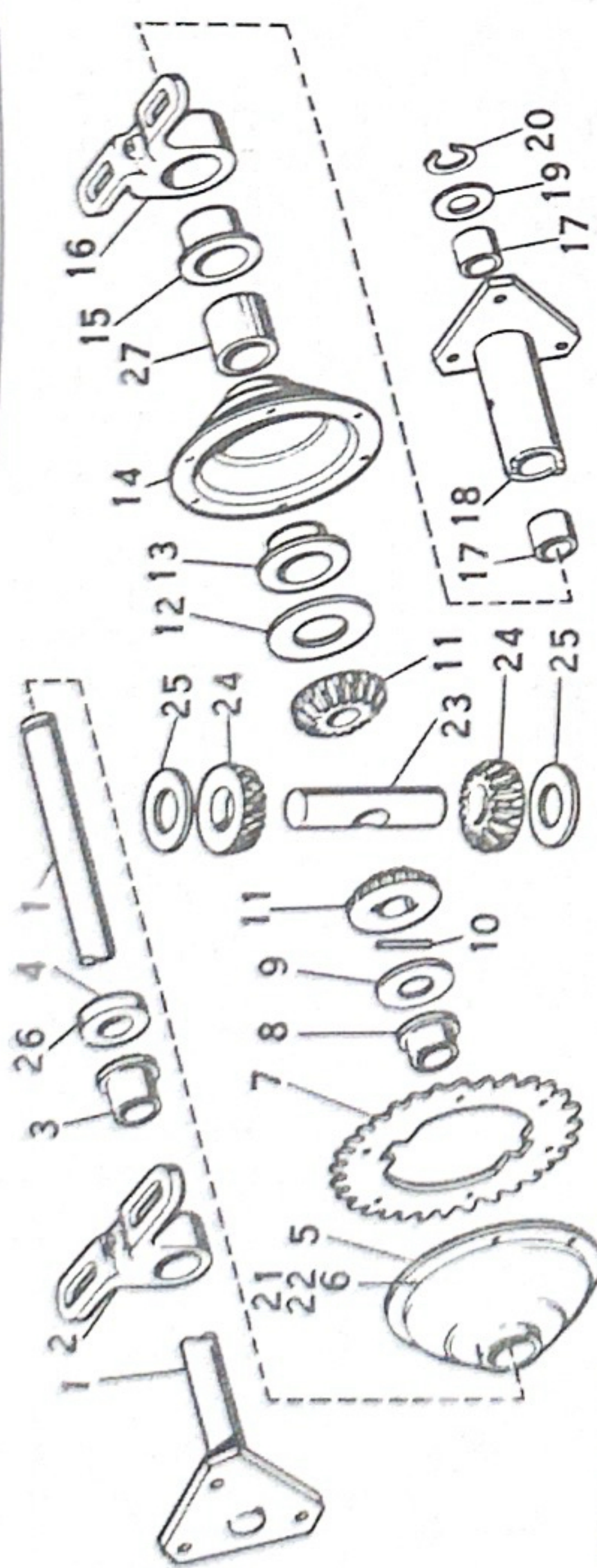
FIGURE 4. REAR AXLE ASSEMBLY
