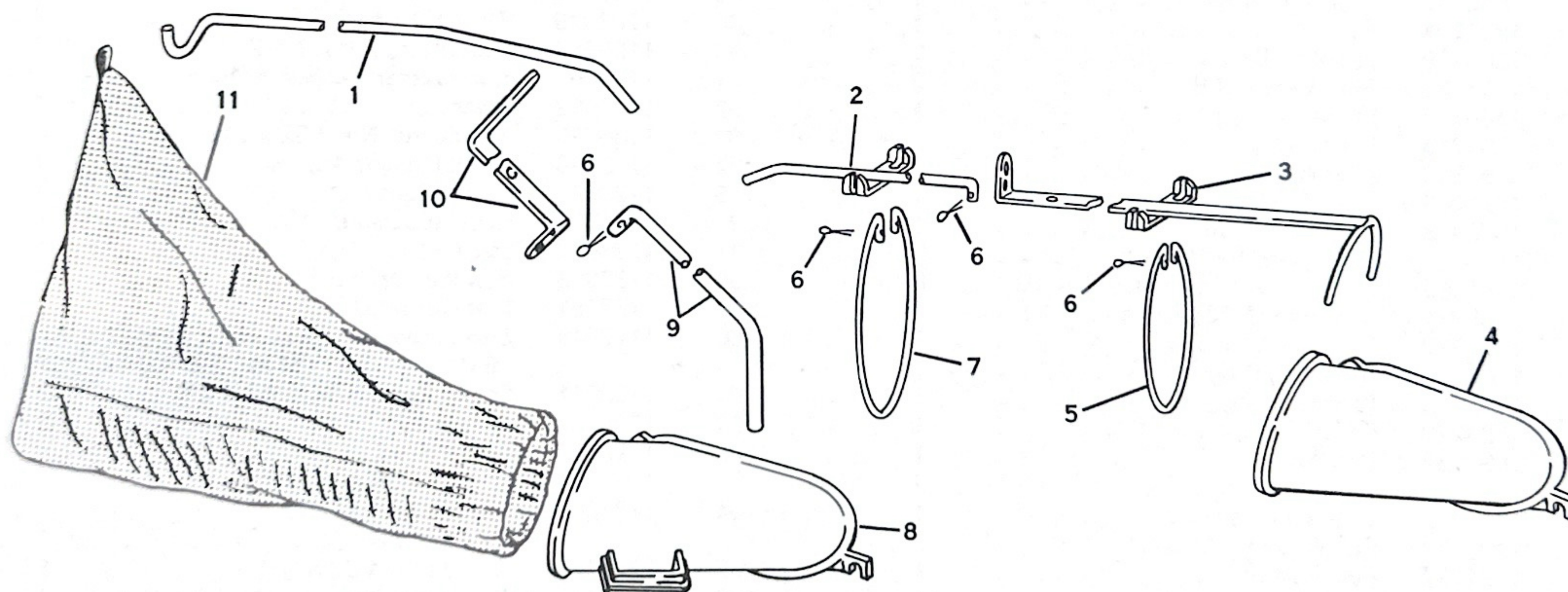
Figure 3 BAG ADAPTER KIT MODELS 6836-01, 6836-02, 6837 & 6838 (Optional)
