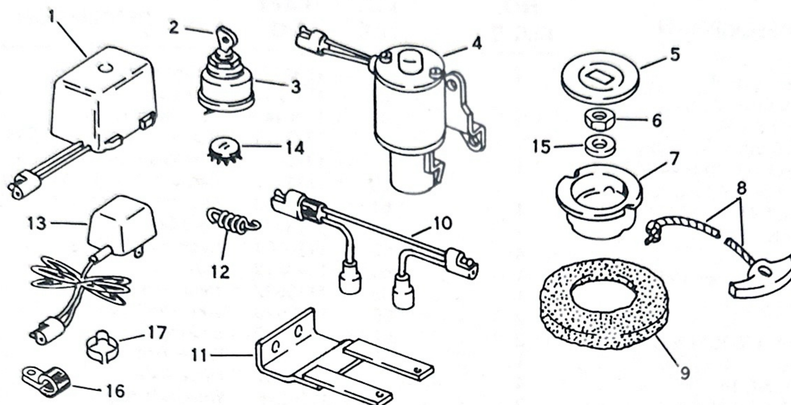
Figure 2 ELECTRIC STARTER KIT MODEL 6839 (Optional)
