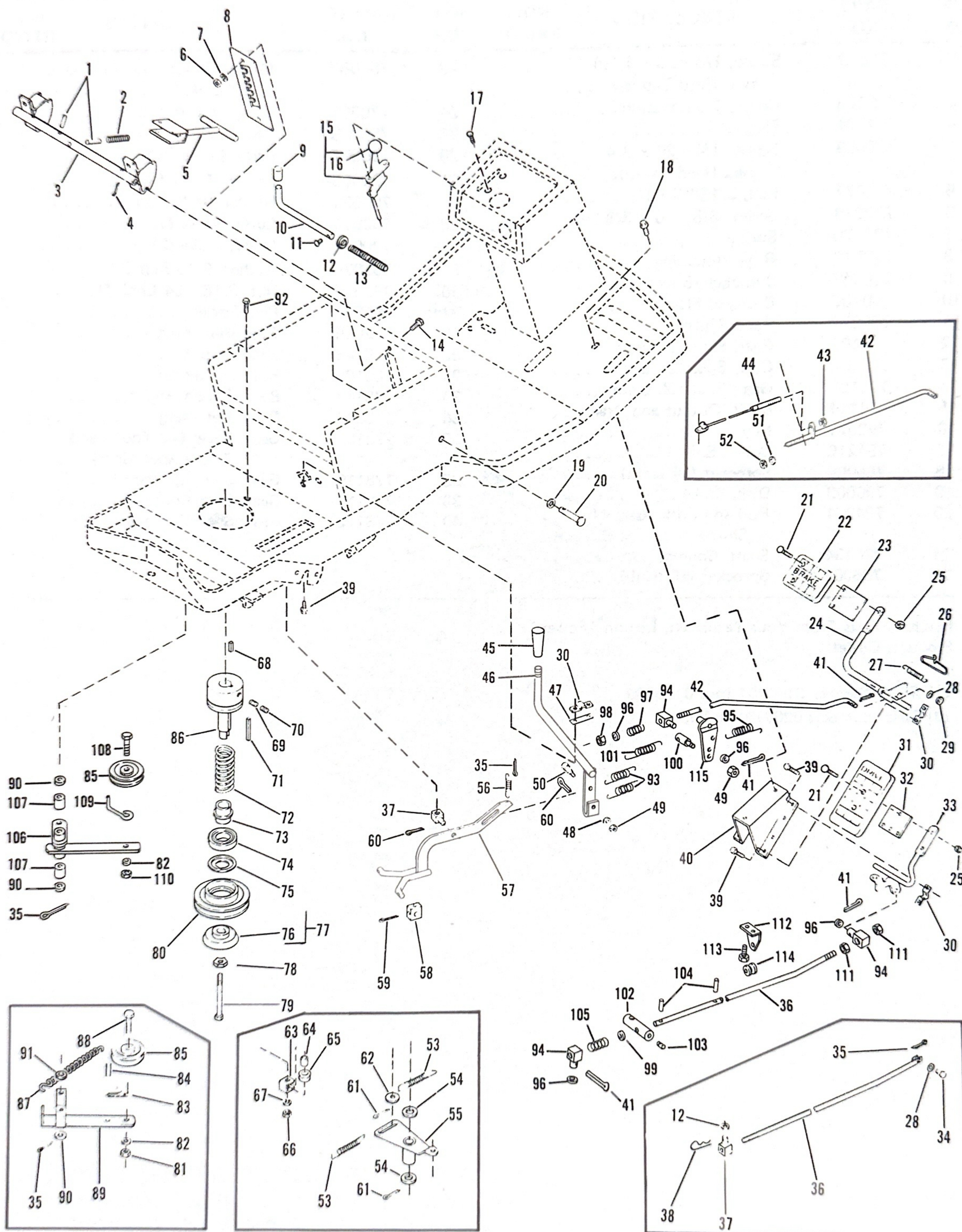
8 Figure 4. HAND CONTROLS, LIFT AND BRAKE CONTROLS
