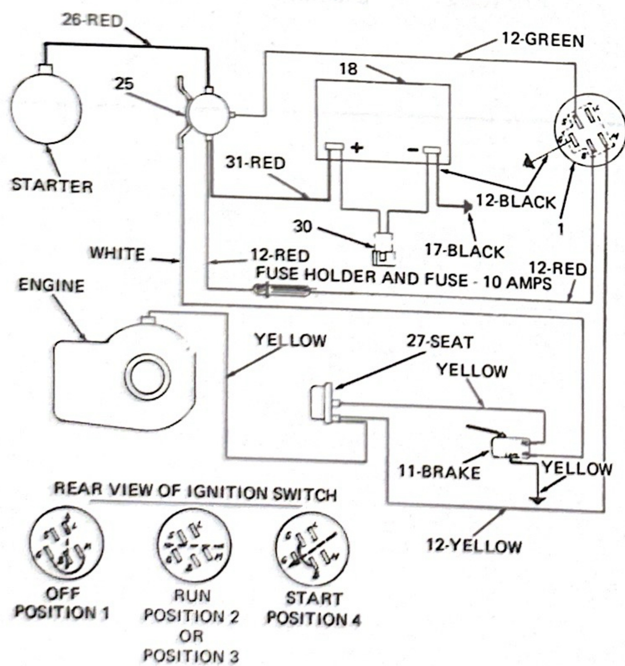
Figure 6. ELECTRICAL SYSTEM
