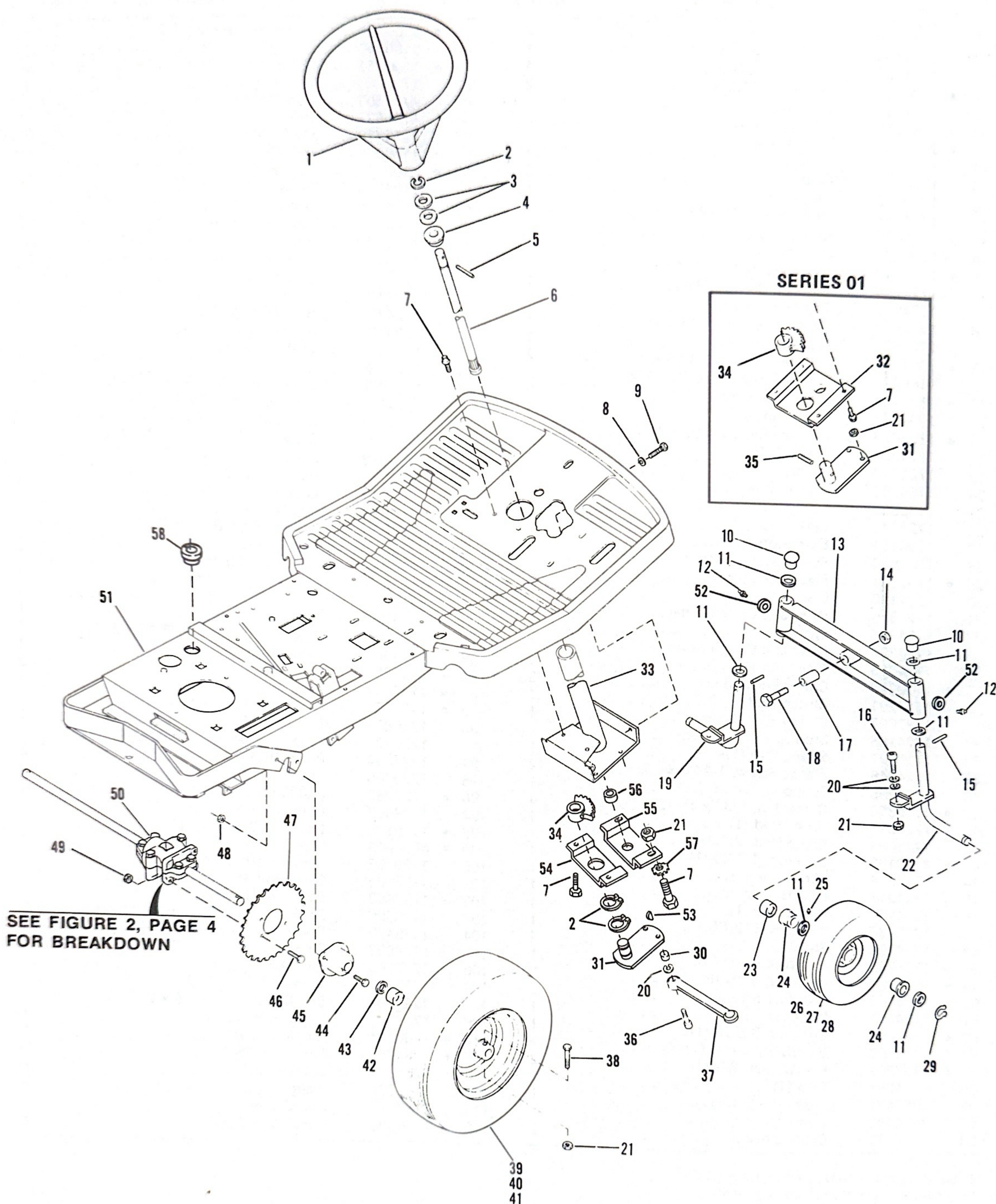
Figure 5. FRAME, STEERING AND AXLE ASSEMBLIES
