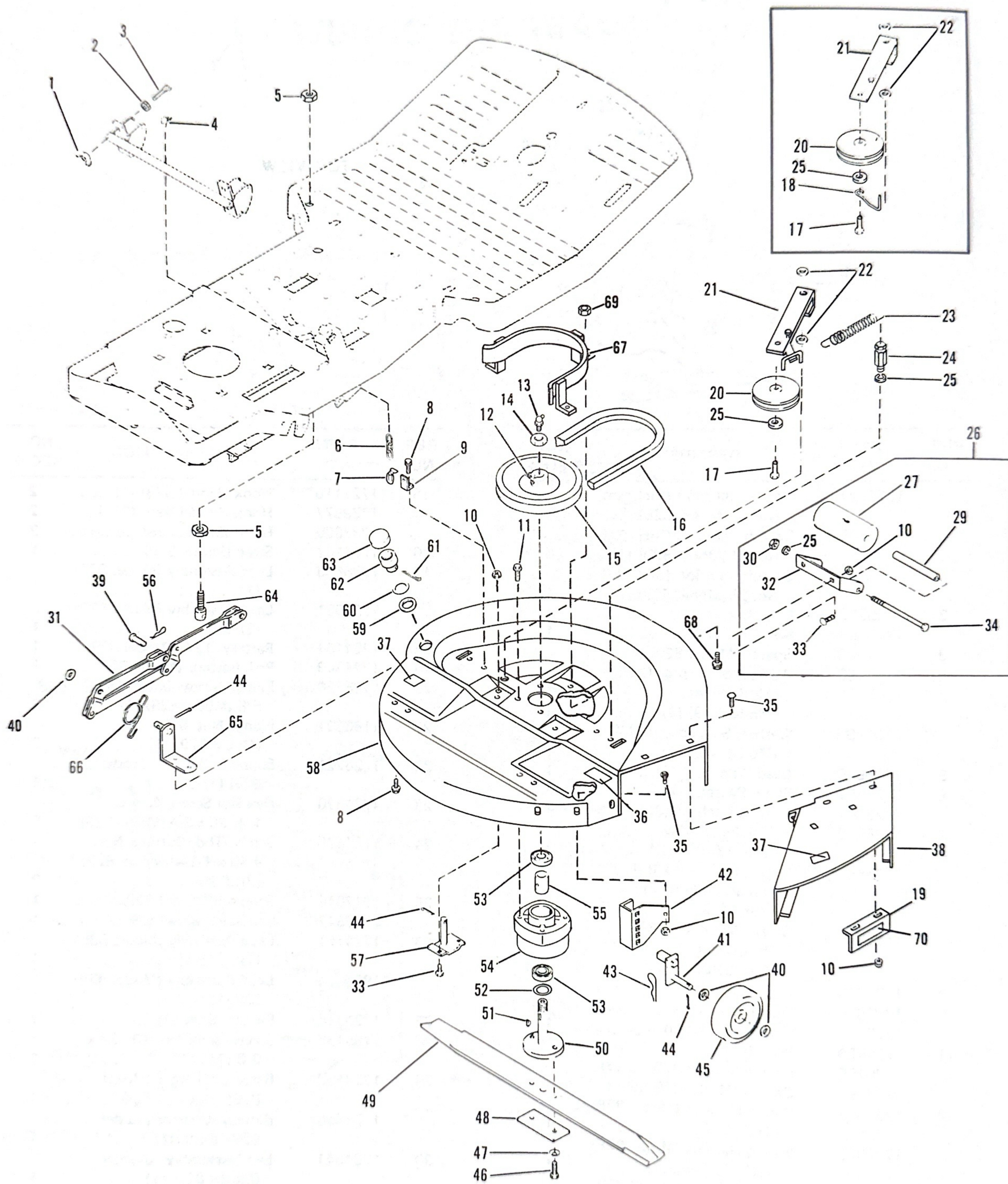
Figure 7. MOWER DECK ASSEMBLY
