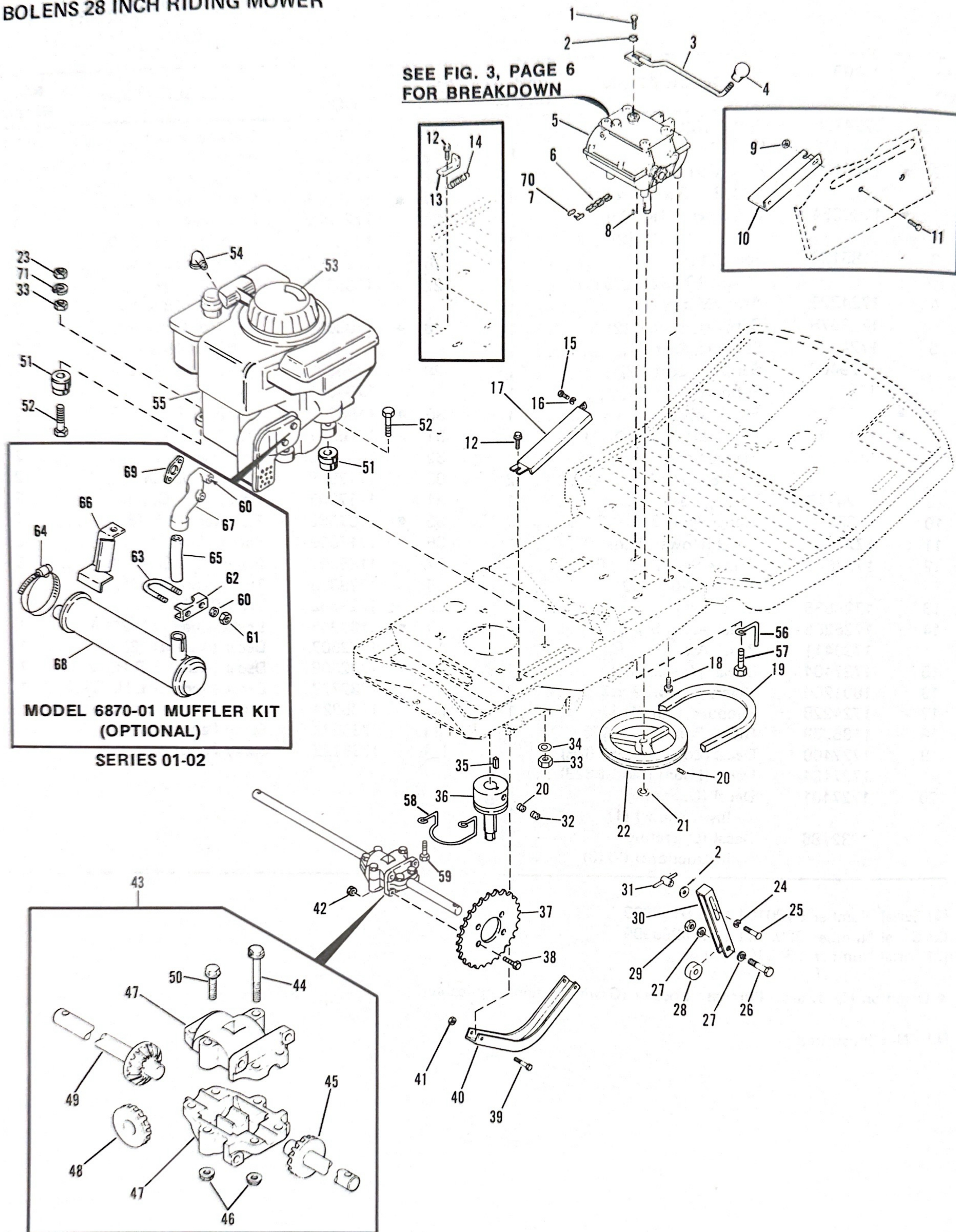
Figure 2. ENGINE AND DRIVE ASSEMBLY
