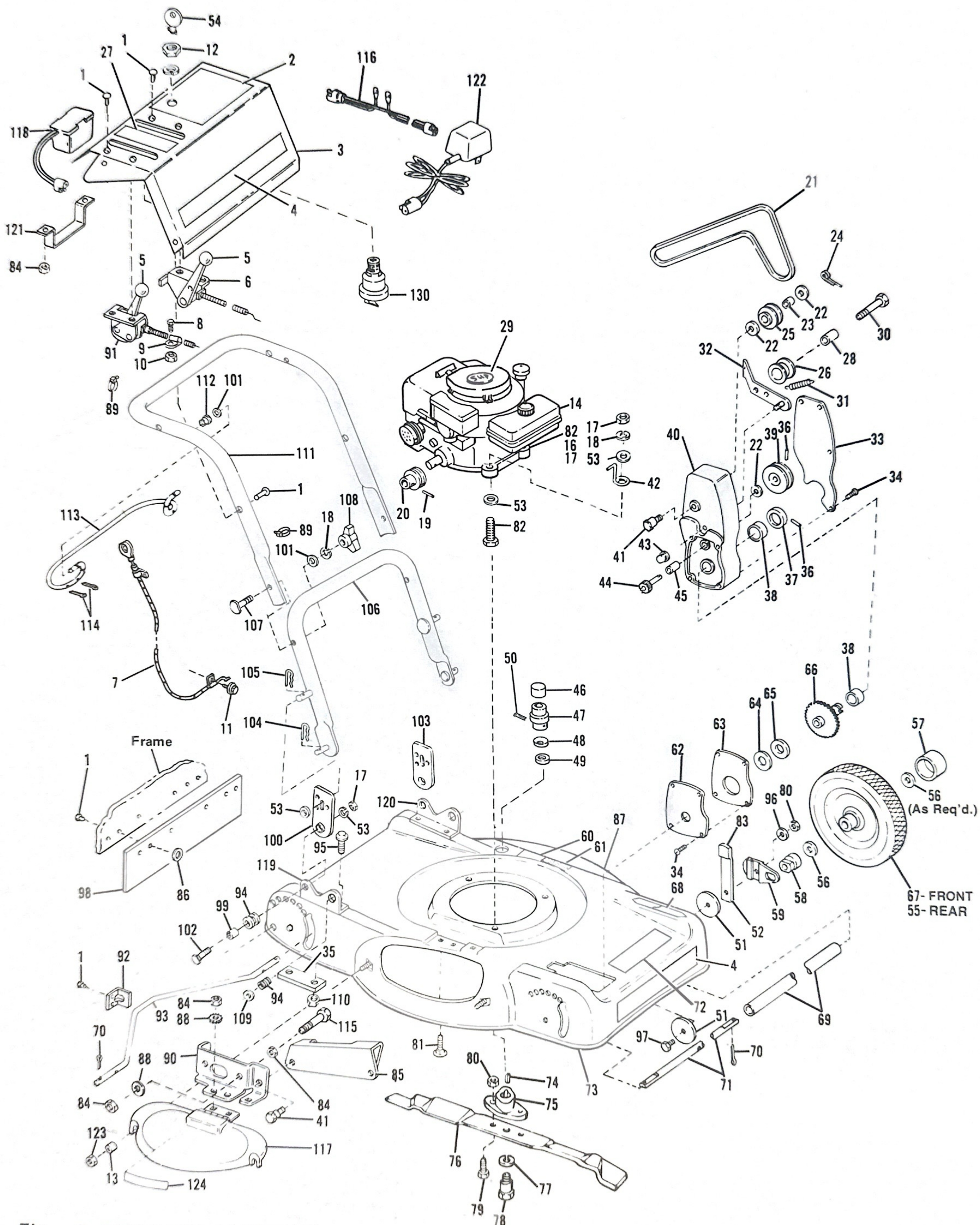
Figure 1 COMPLETE ASSEMBLY
