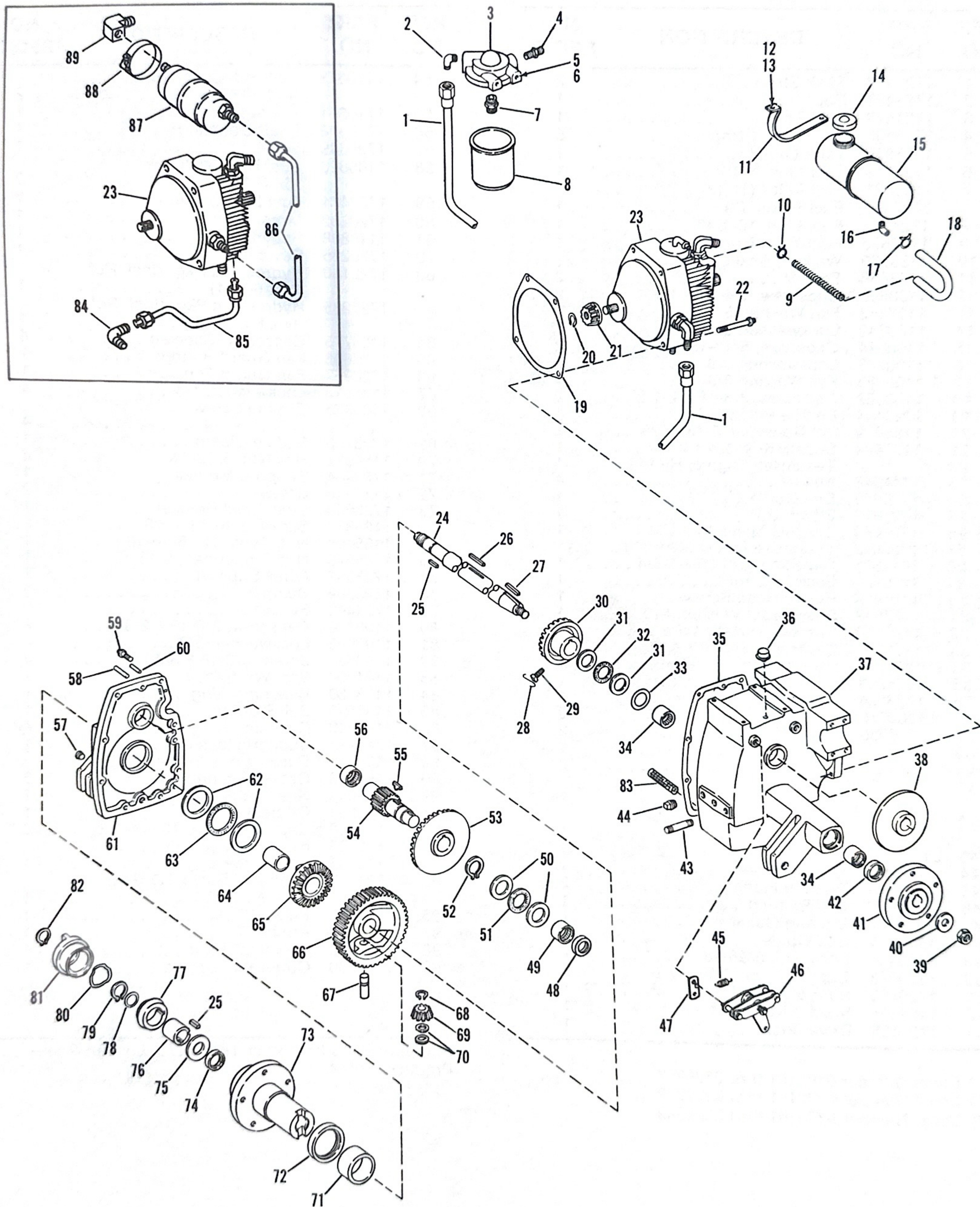
Figure 3 HYDRO AND TRANSAXLE ASSEMBLY
