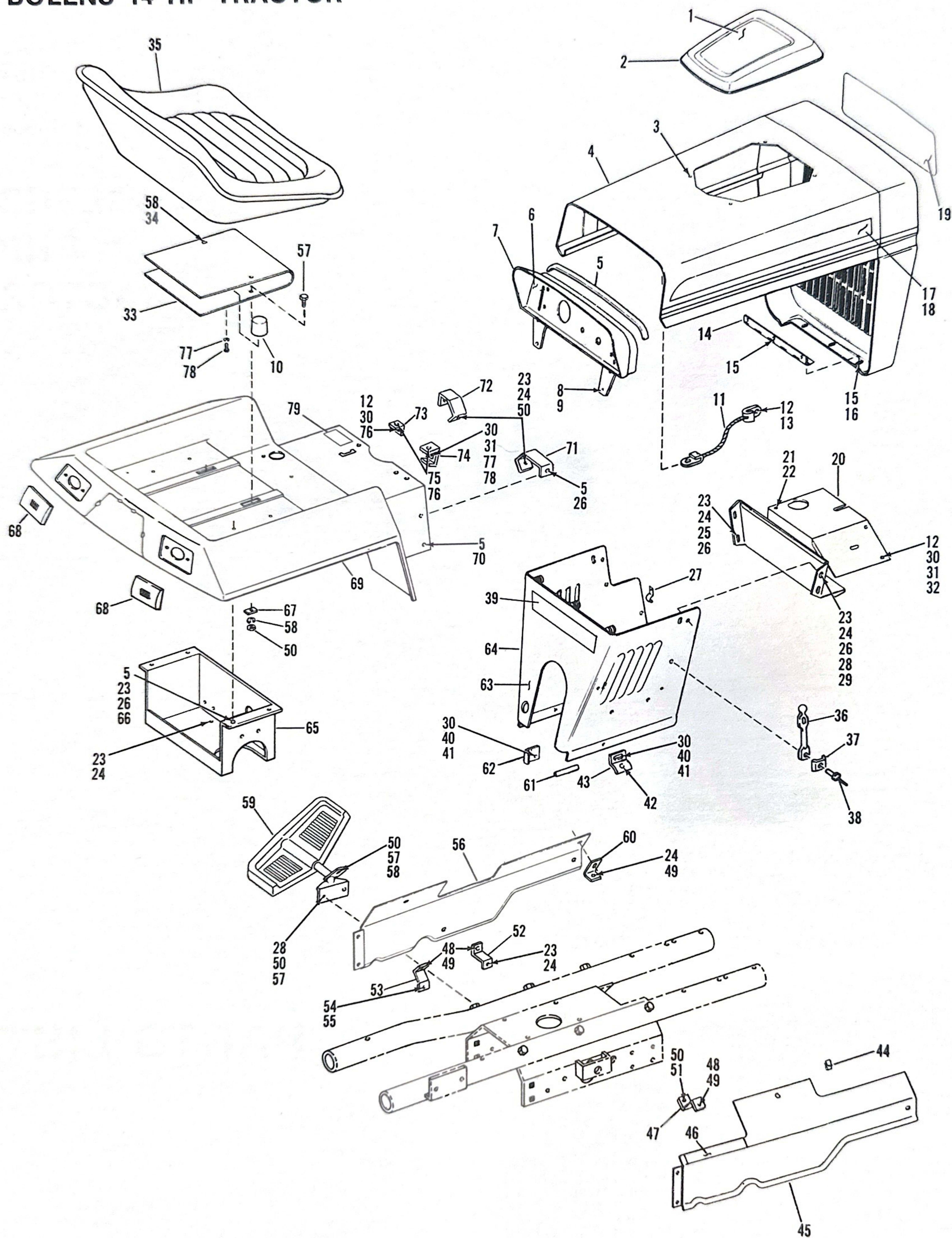
Figure 1 TRIM ASSEMBLY
