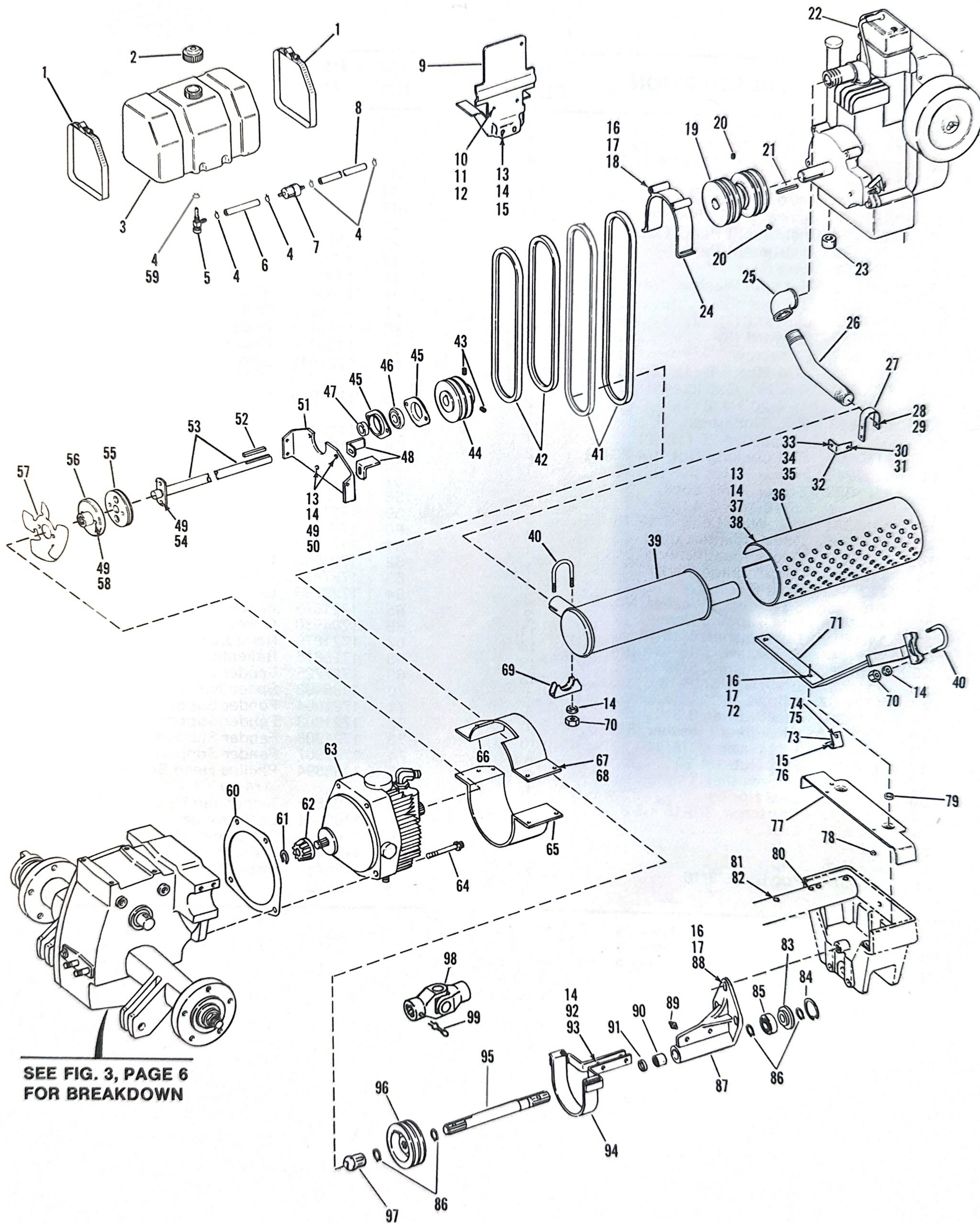
Figure 2 ENGINE AND DRIVE ASSEMBLY
