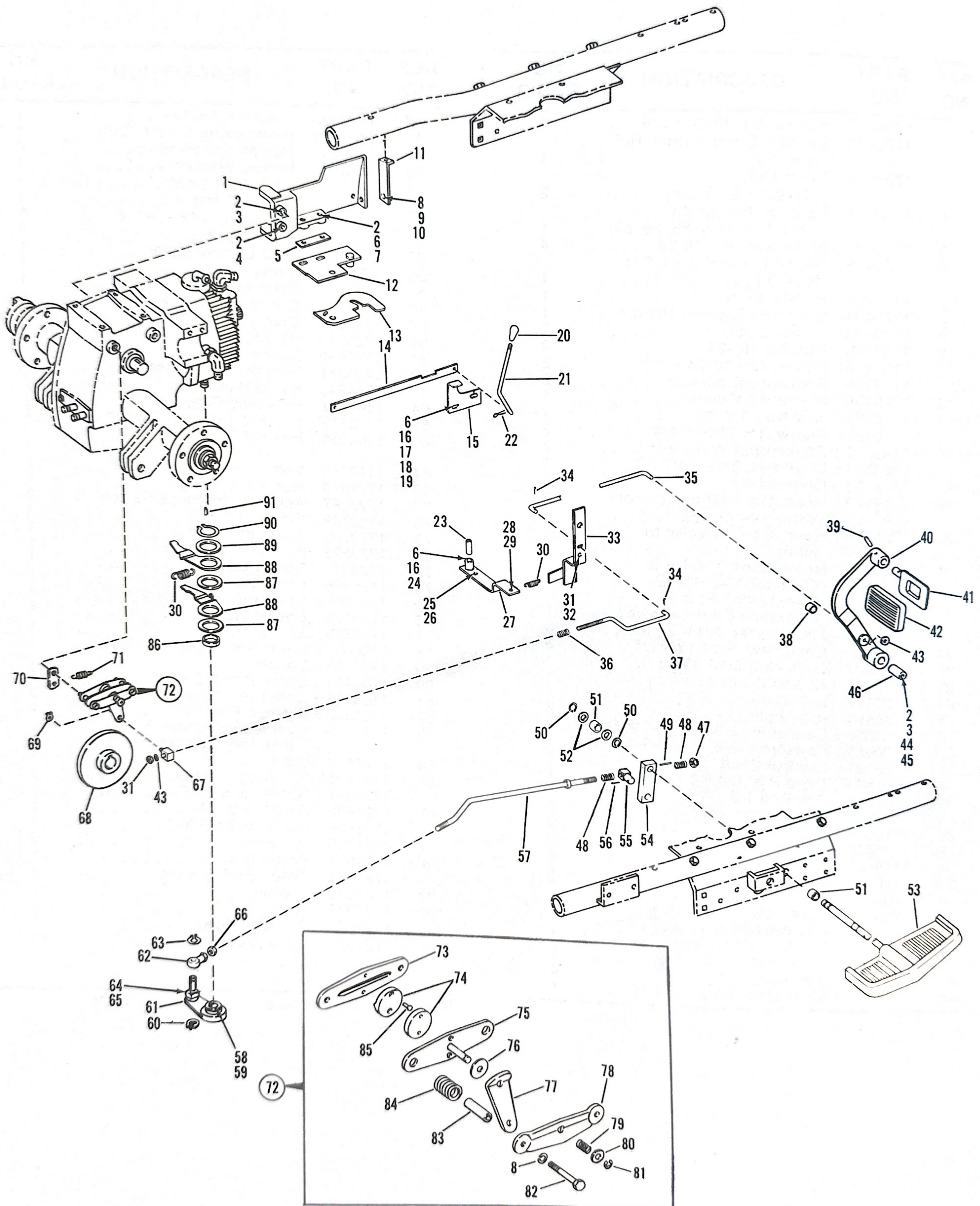
Figure 5 BRAKE AND HYDRO CONTROL ASSEMBLIES
