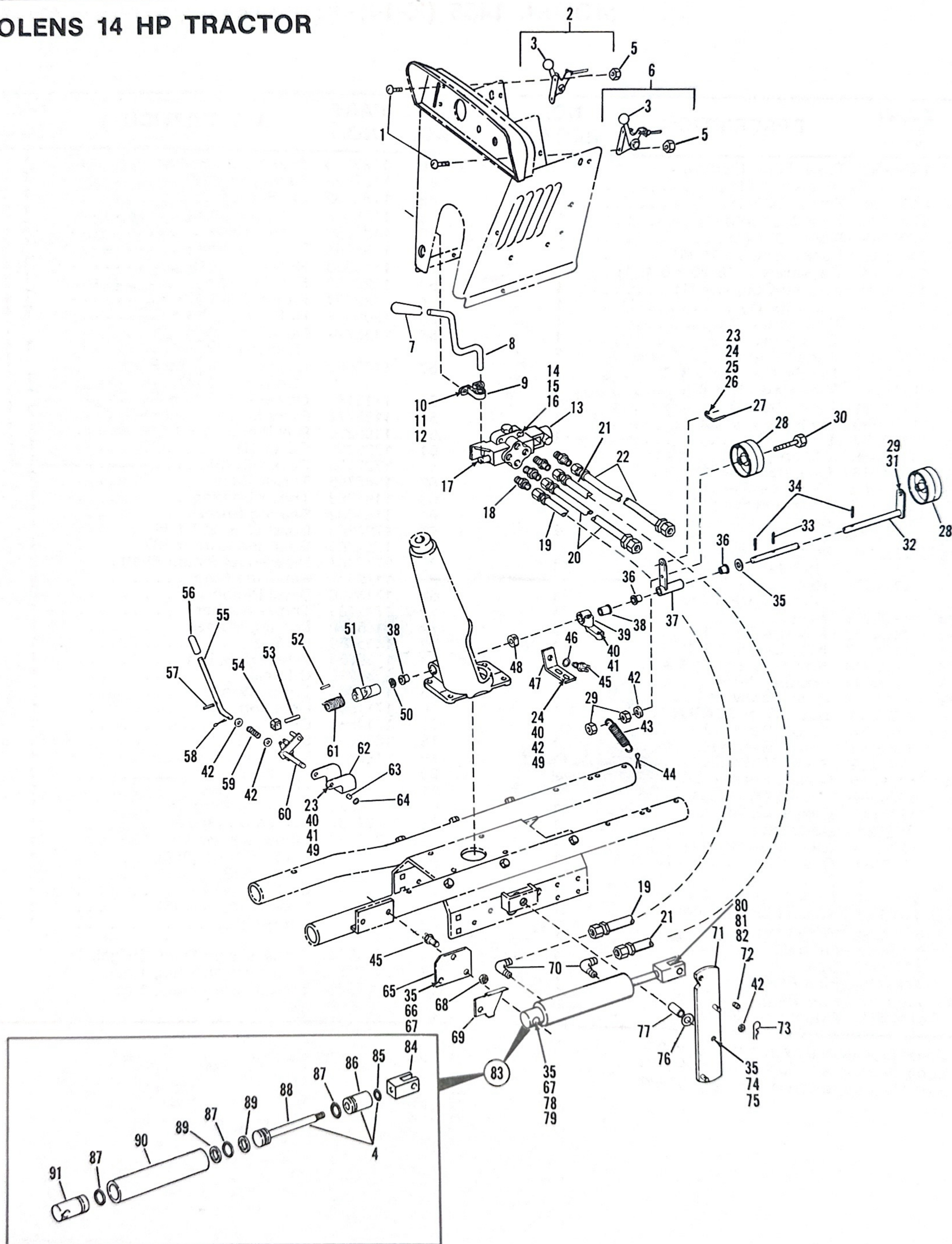
Figure 4 HAND CONTROLS AND LIFT ASSEMBLY
