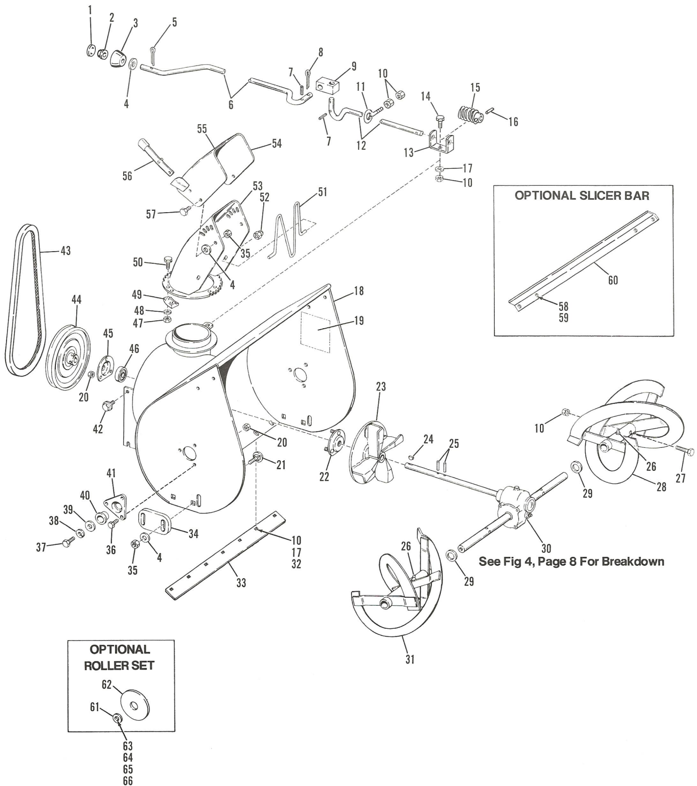
Figure 3 BLOWER HOUSING ASSEMBLY
